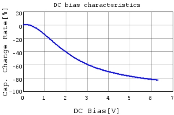
GRM21BR60J107ME15 C-DC bias capchange, 25.0c
