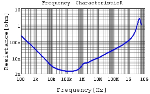
GRM21BR60J107ME15 R DCOV, 25degC
