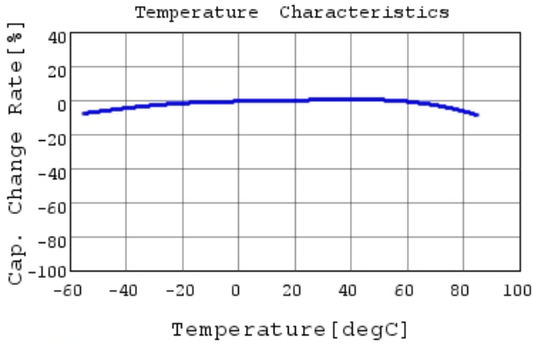
GRM21BR60J107ME15 C-Temp. capchange, DC0.0V,
