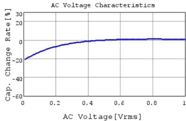
GRM21BR60J107ME15 C-AC Voltage capchange, Dc
