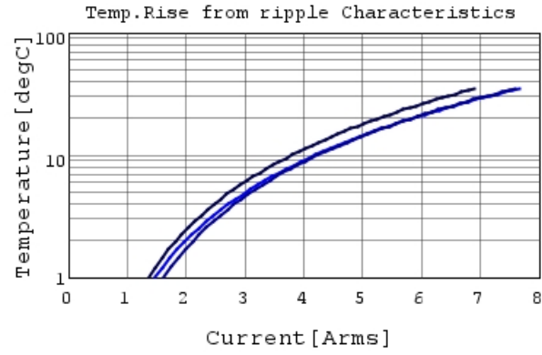
GRM31CR60J227ME11 Temp.rise — 50kHz
