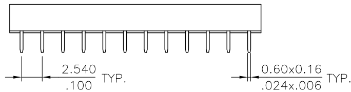
Typical 24,28 Circuits
