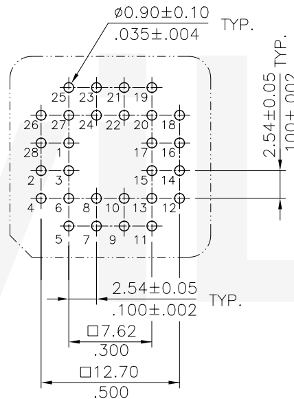
Recommended P.C. Board Layout
