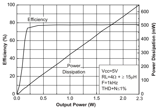
Figure 8. Efficiency vs. output power
