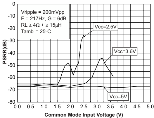
Figure 20. PSRR vs. common mode input voltage
