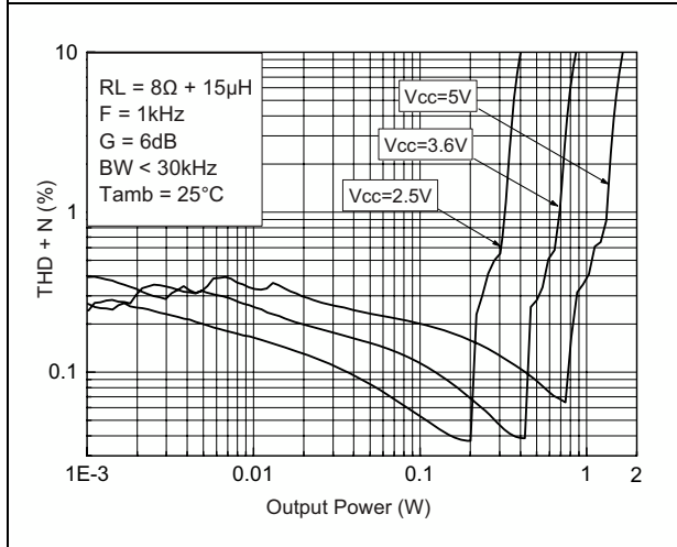
Figure 34. THD+N vs. output power
