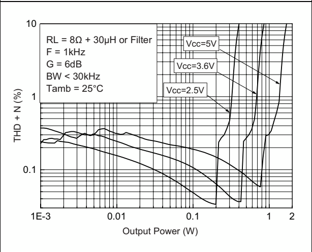
Figure 35. THD+N vs. output power
