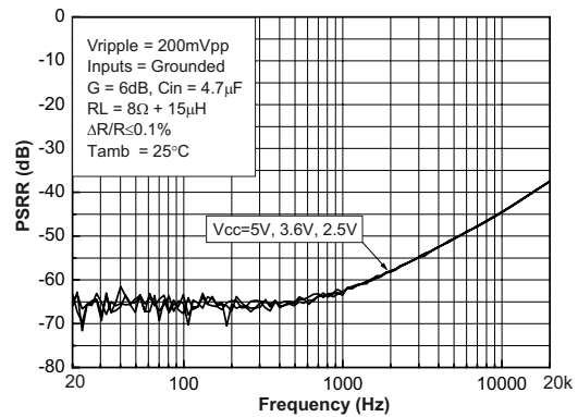
Figure 19. PSRR vs. frequency
