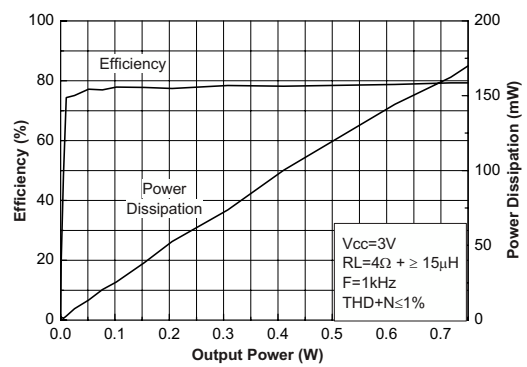
Figure 9. Efficiency vs. output power
