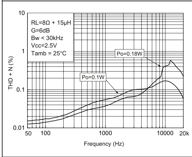
Figure 46. THD+N vs. frequency
