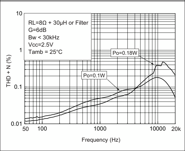
Figure 47. THD+N vs. frequency
