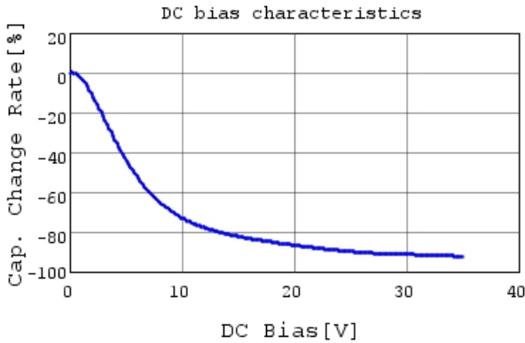
GRM188R6YA475KE15 C-DC bias capchange, 25.0c
