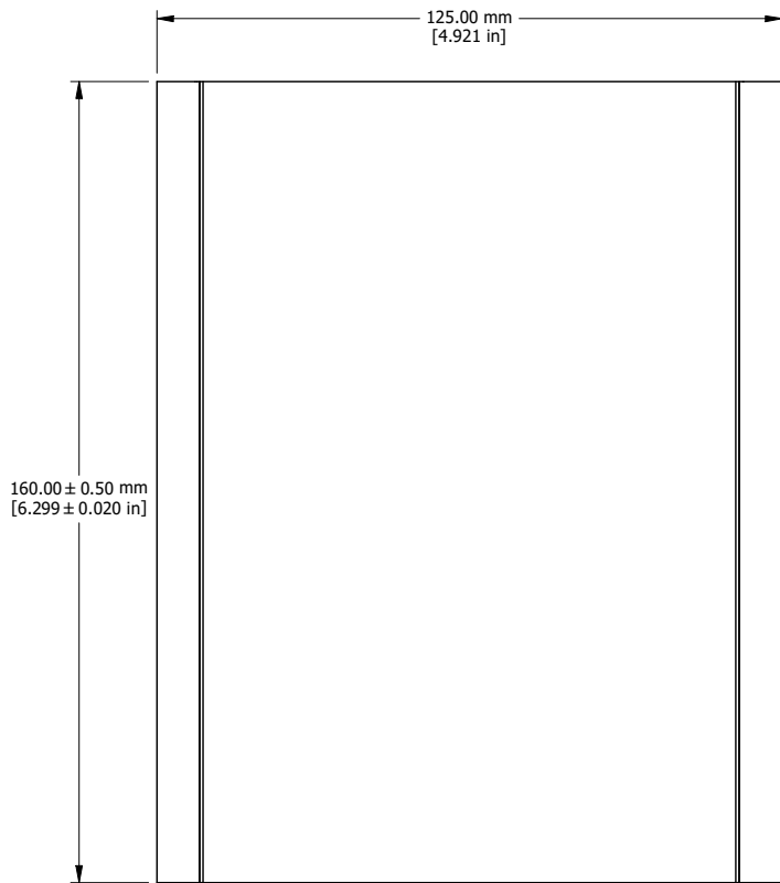
EXTRUSION
