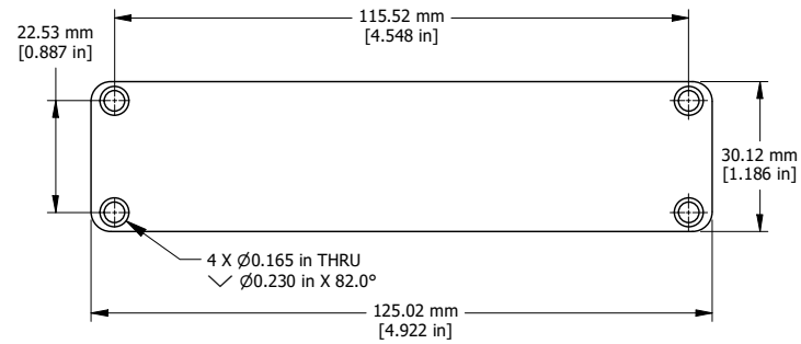
OPTIONAL FLANGE END PANELS 1455PF
