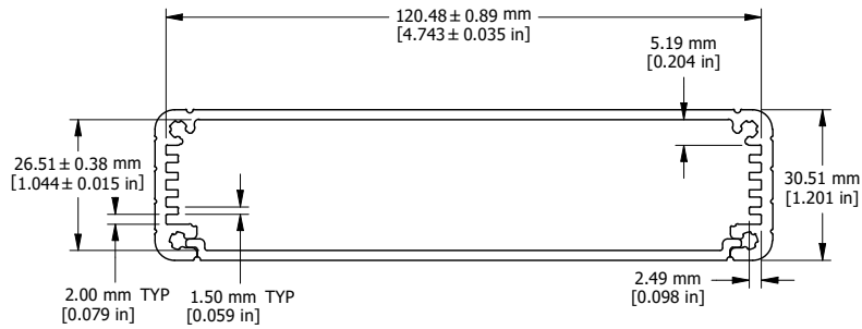
EXTRUSION
