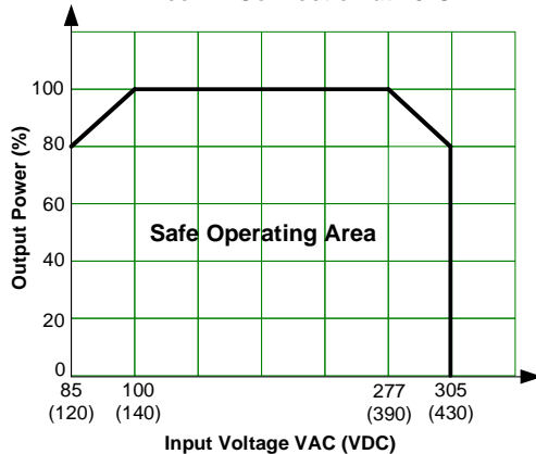
Free Air Convection at 25°C
