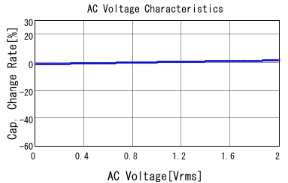
■ GRM188R72A221KA01 C-AC Voltage capchange, DCOV, 25.0d
