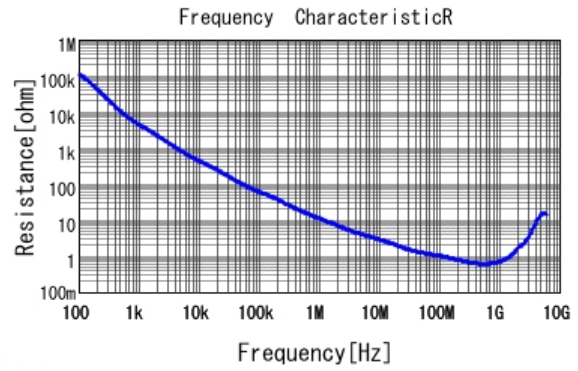
■ GRM188R72A221KA01 R DCOV, 25degC
