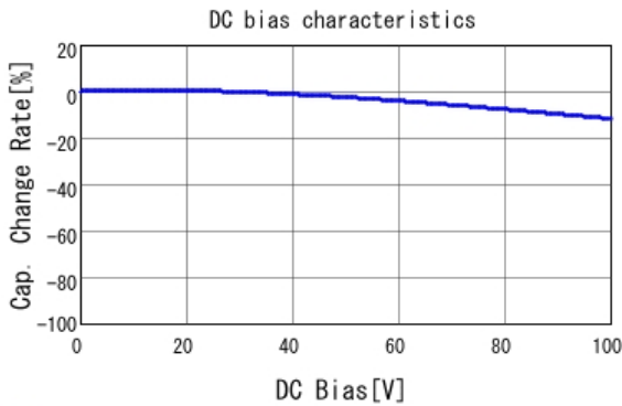
■ GRM188R72A221KA01 C-DC bias capchange, 25.0degC, AC1.
