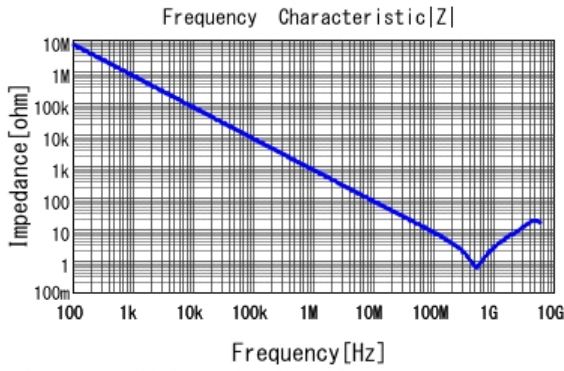
■ GRM188R72A221KA01 |Z| DCOV, 25degC
