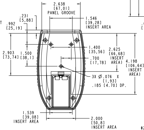
BOTTOM COVER - INTERIOR VIEW
