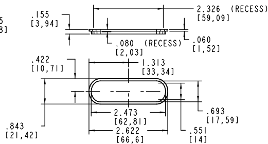
BOTTOM COVER - INTERIOR VIEW
