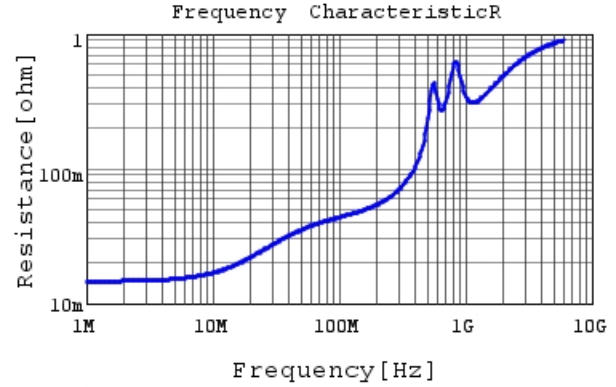
GRM1555C1H102JA01 R DCOV, 25degC
