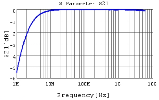
GRM1555C1H102JA01 S21 DCOV, 25degC
