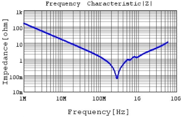
GRM1555C1H102JA01 |Z| DCOV, 25degC
