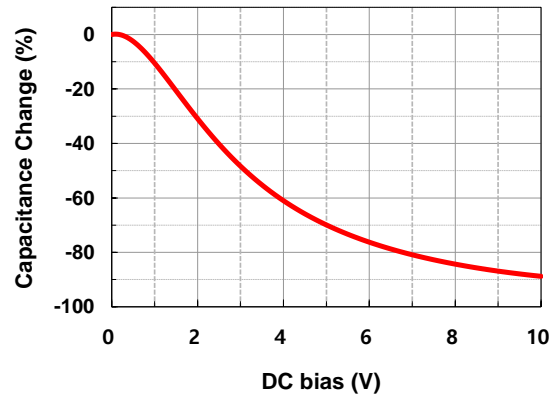
- Capacitance Change(%) with DC bias
