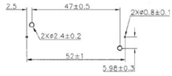
PCB/MOUNTING LAYOUT
