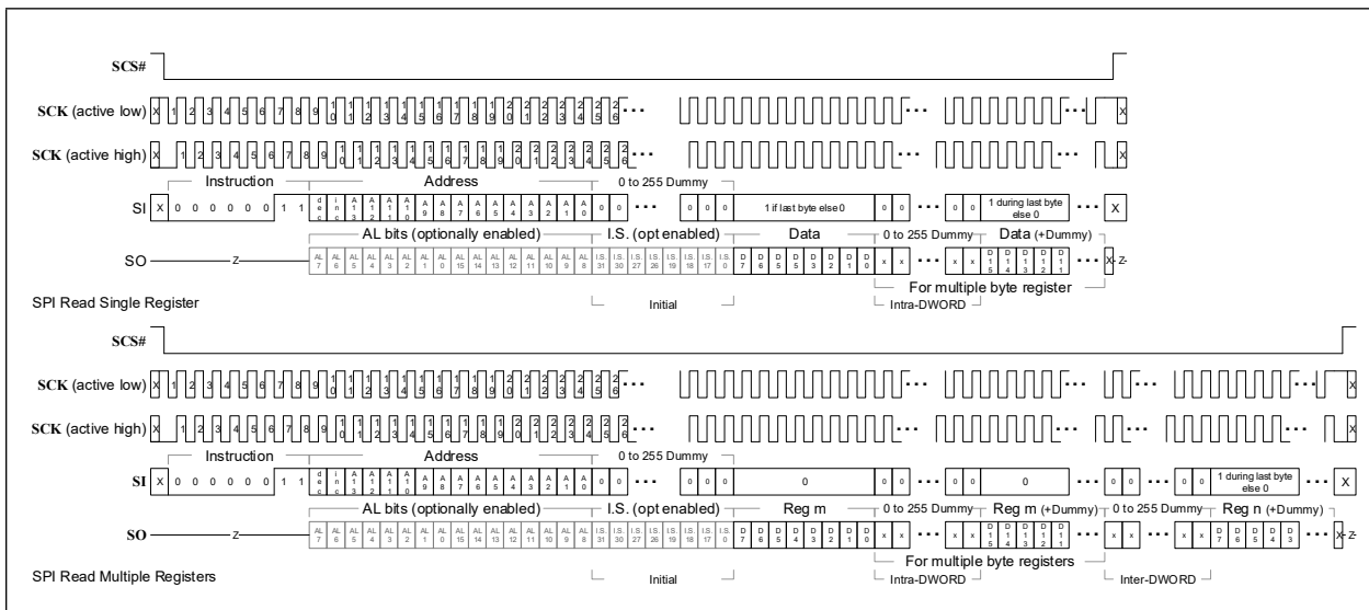
FIGURE 9-6: SPI READ
