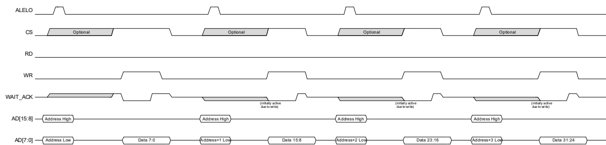
FIGURE 8-44: MULTIPLYED ADDRESSING WITH SINGLE PHASE LATCHING - 8-BIT NON-POSTED WRITE
