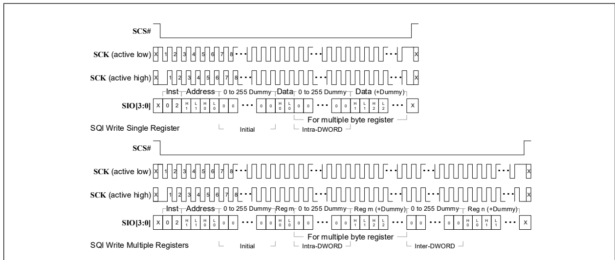
FIGURE 9-14: SQI WRITE
