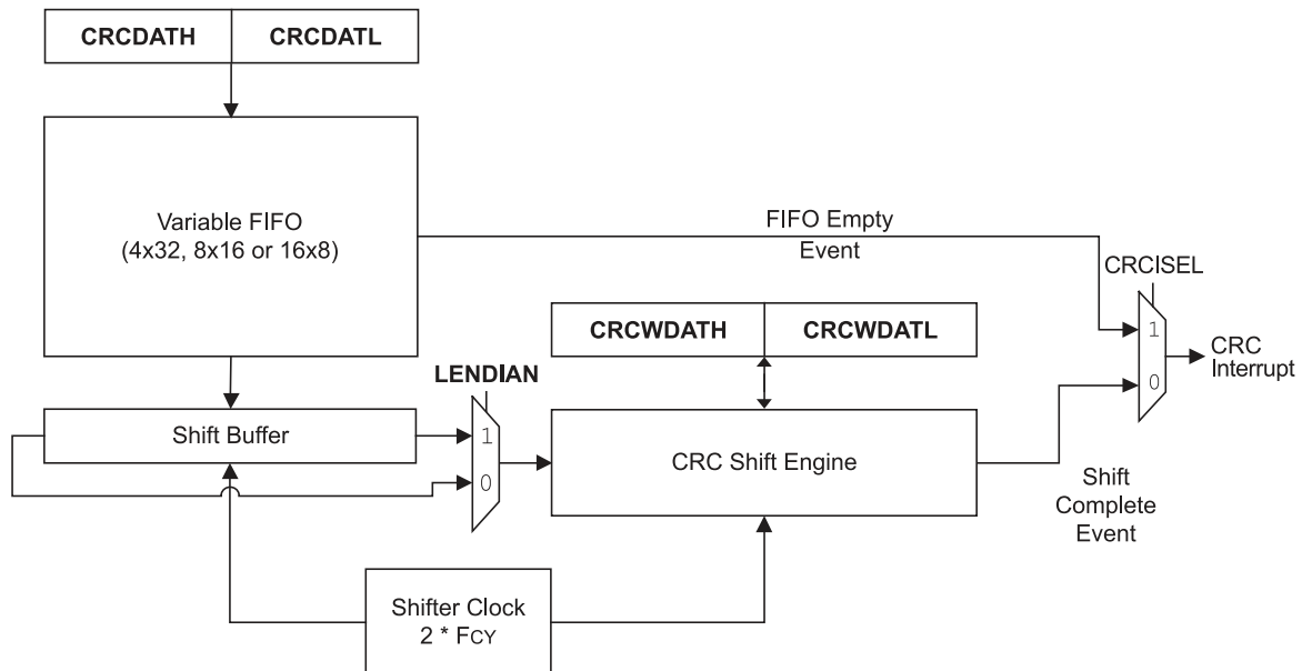
Figure 19-2. CRC Shift Engine Detail
