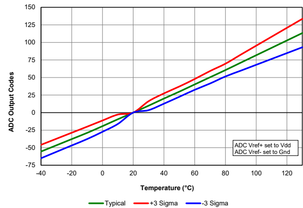
Figure 40-88. Temperature Indicator, Slope Normalized to 20°C, High Range, V DD = 5.5V, PIC18F67K40 only
