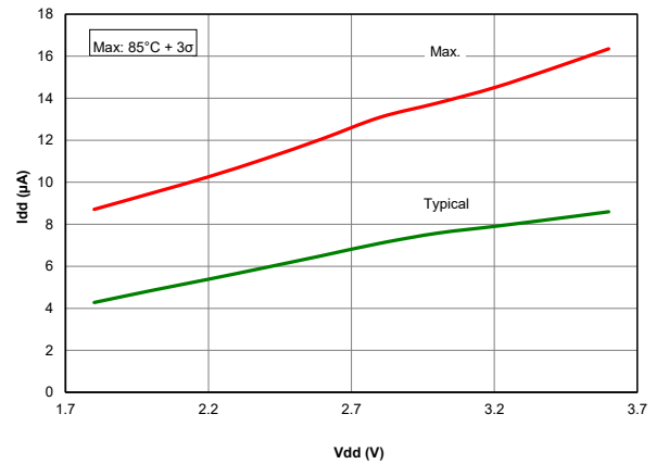
Figure 40-48. I_{DD} , LFINTOSC, F_{OSC} = 31kHz , PIC18LF67K40 only
