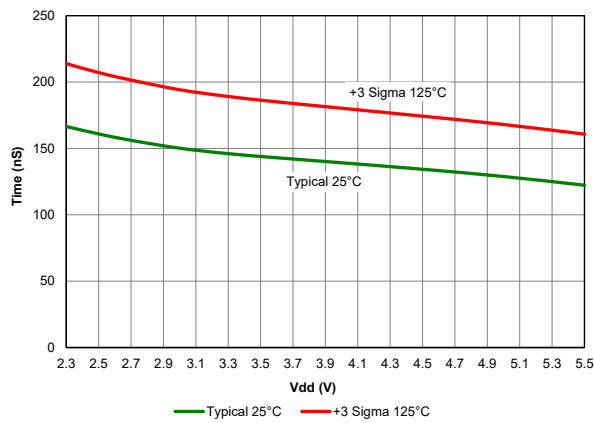
Figure 40-25. Comparator Response Time, Falling Edge, PIC18F67K40 only
