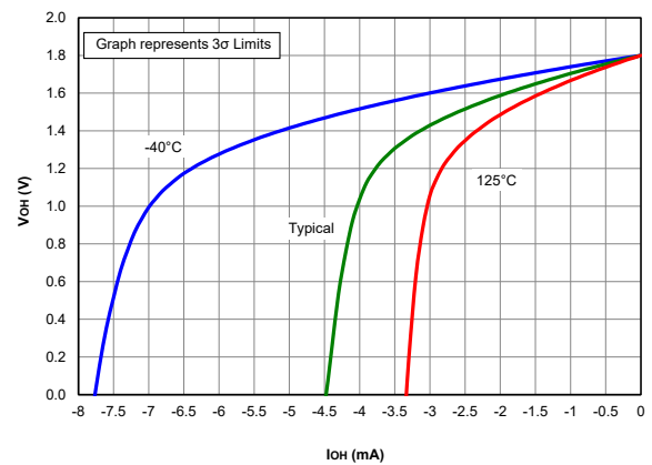
Figure 40-98. V_{OH} vs I_{OH} , Over Temperature, V_{DD} = 5.0V , PIC18LF67K40 only
