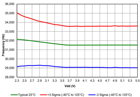
Figure 40-77. LFINTOSC Frequency, PIC18F67K40 only
