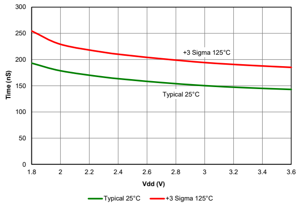
Figure 40-23. Comparator Response Time, Falling Edge, PIC18LF67K40 only
