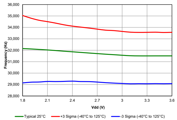
Figure 40-76. LFINTOSC Frequency, PIC18LF67K40 only
