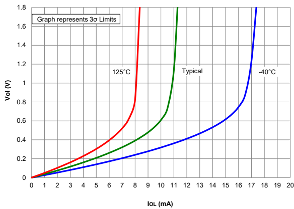
Figure 40-99. V_{OL} vs I_{OL} , Over Temperature, V_{DD} = 5.0V , PIC18LF67K40 only
