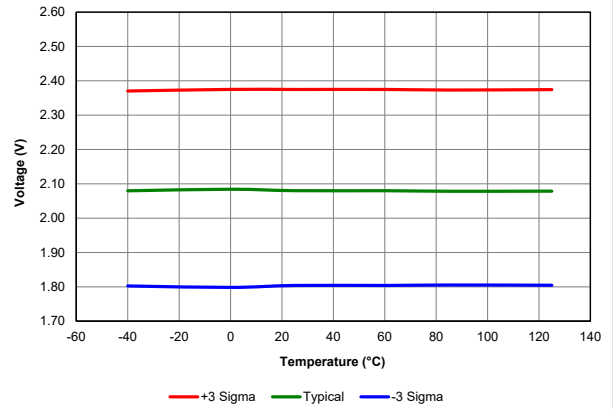
Figure 40-17. LPBOR Reset Voltage, PIC18LF67K40 only
