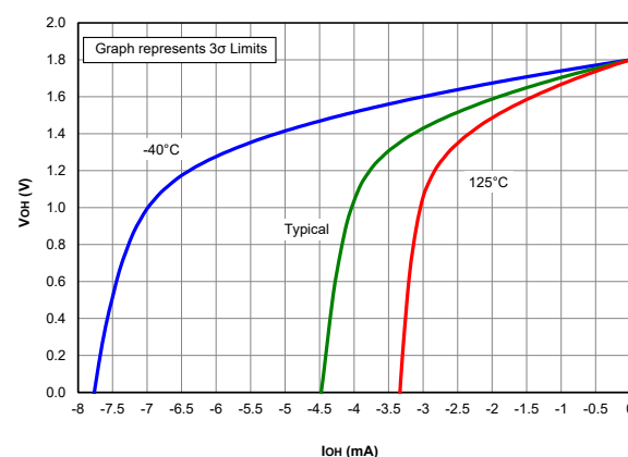
Figure 40-98. V_{OH} vs I_{OH} , Over Temperature, V_{DD} = 5.0V , PIC18LF67K40 only
