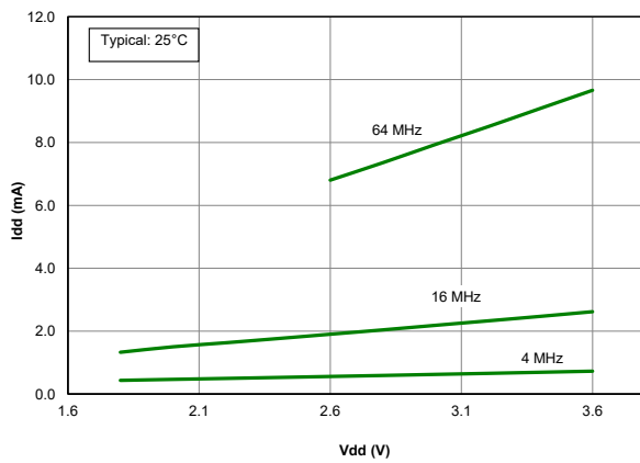
Figure 40-53. I_{DD} , HFINTOSC, Typical, PIC18LF67K40 only
