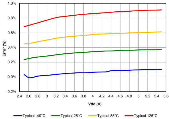
Figure 40-37. Typical FVR Voltage Error 2x, PIC18F67K40 only
