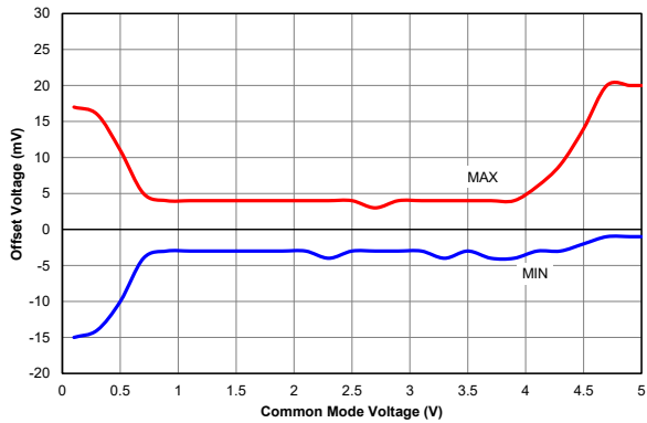
Figure 40-31. Comparator Offset, V_{DD} = 5.0V , 25^{\circ}C , PIC18F67K40 only
