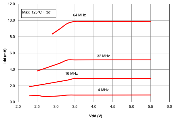
Figure 40-43. I_{DD} Maximum, HFINTOSC, PIC18F67K40 only
