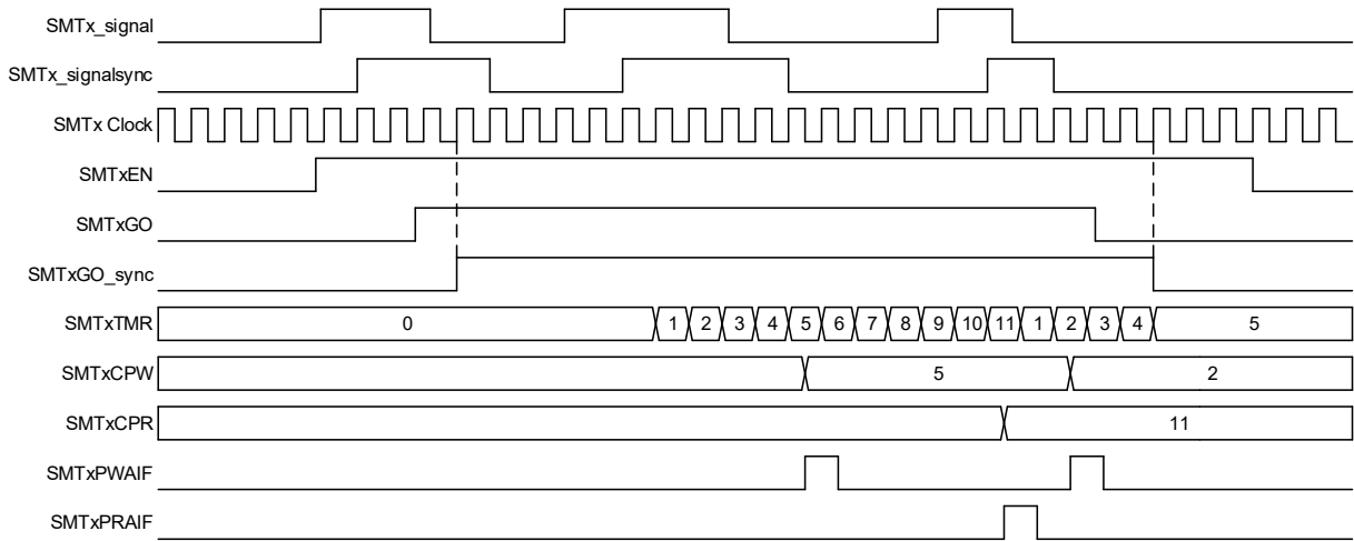
Figure 25-6. Period and Duty Cycle, Single Acquisition Mode Timing Diagram
