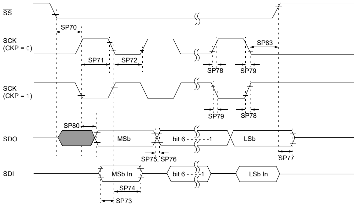
Figure 39-18. SPI Client Mode Timing (CKE = 0)
