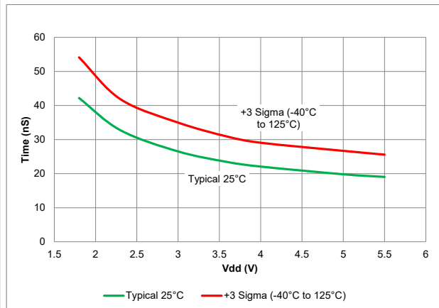
Figure 40-58. I/O Fall Time, Slew Rate Control Enabled
