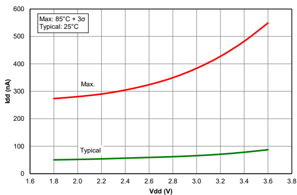
Figure 40-71. I_{PD} Base, Low-power Sleep Mode, PIC18LF67K40 only
