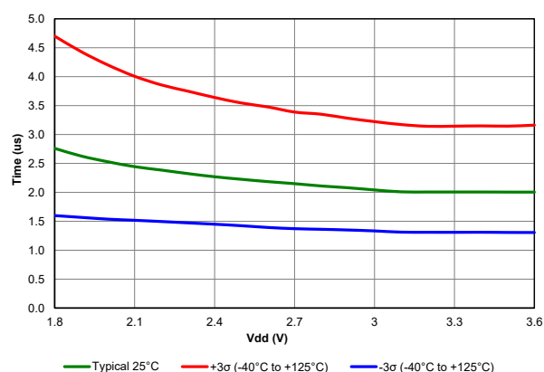
Figure 40-9. ADC RC Oscillator Period, PIC18LF67K40 only
