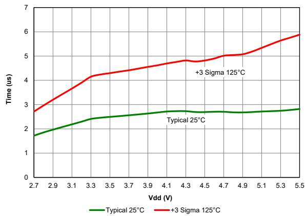
Figure 40-22. BOR Response Time, PIC18F67K40 only
