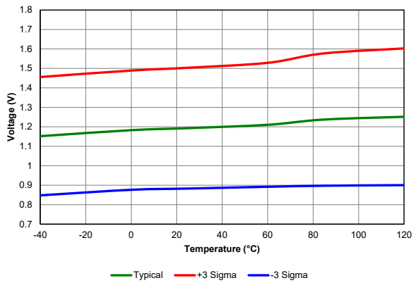
Figure 40-81. POR Rearm Voltage, VREGPM1 = 1, PIC18F67K40 only
