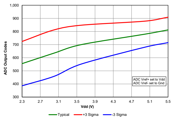
Figure 40-86. Temperature Indicator, Initial Offset, Low Range, Temp = 20°C, PIC18F67K40 only
