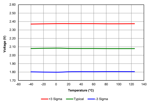
Figure 40-17. LPBOR Reset Voltage, PIC18LF67K40 only
