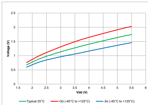
Figure 40-55. Schmitt Trigger Low Values
