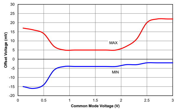
Figure 40-28. Comparator Offset, V_{DD} = 3.0V , from -40^{\circ}C to 125^{\circ}C
