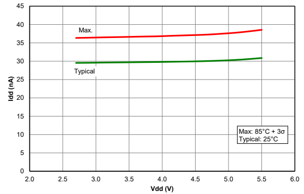
Figure 40-64. I_{PD} , Fixed Voltage Reference (FVR), PIC18F67K40 only
