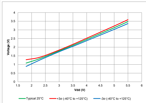
Figure 40-54. Schmitt Trigger High Values
