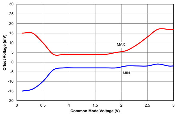
Figure 40-27. Comparator Offset, V_{DD} = 3.0V , 25^{\circ}C
