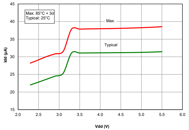
Figure 40-42. I DD , LFINTOSC, F OSC = 31kHz, PIC18F67K40 only
