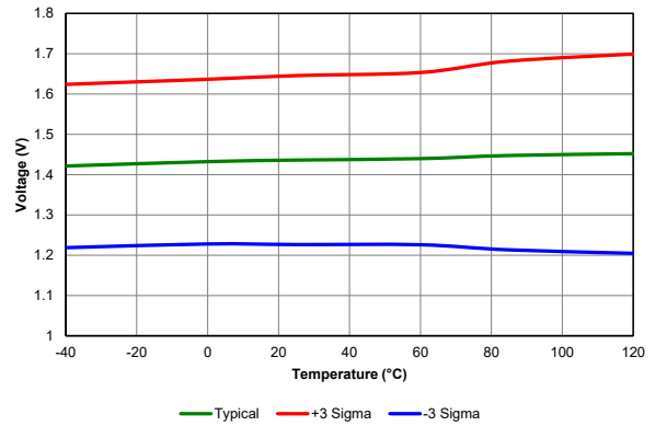
Figure 40-80. POR Rearm Voltage, VREGPM1 = 0, PIC18F67K40 only
