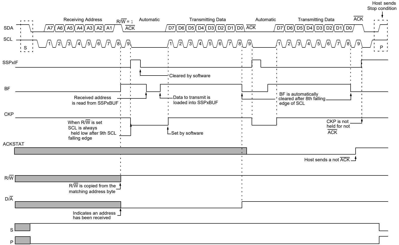
Figure 27-18. I 2 C Client, 7-Bit Address, Transmission (AHEN = 0)
