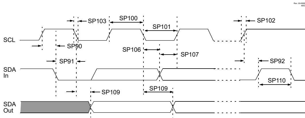
Figure 39-21. I 2 C Bus Data Timing
