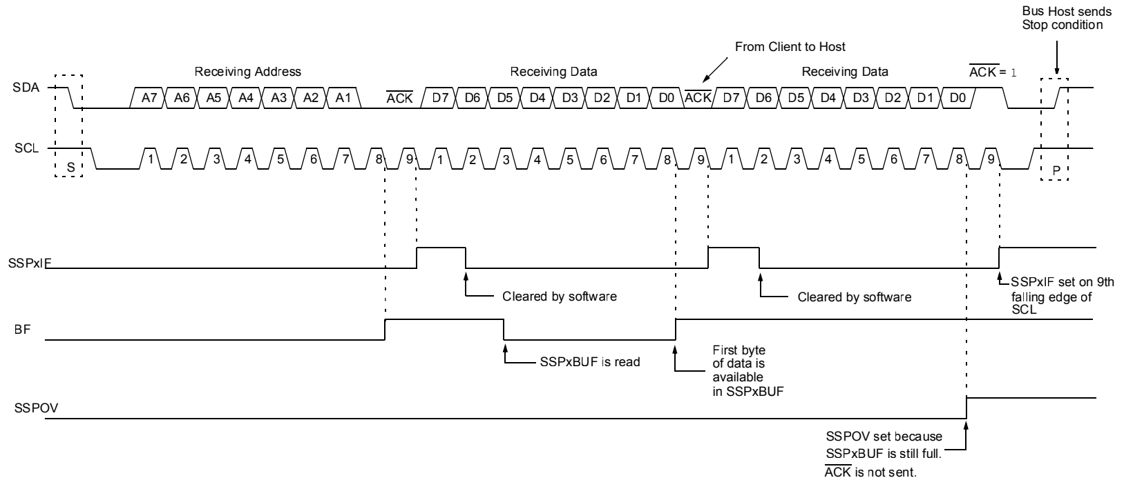
Figure 27-14. I 2 C Client, 7-Bit Address, Reception (SEN = 0, AHEN = 0, DHEN = 0)
