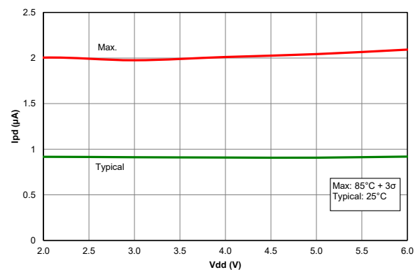
Figure 40-62. I PD , Watchdog Timer, PIC18F67K40 only
