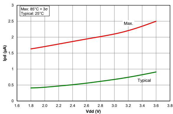
Figure 40-61. I PD , Watchdog Timer, PIC18LF67K40 only
