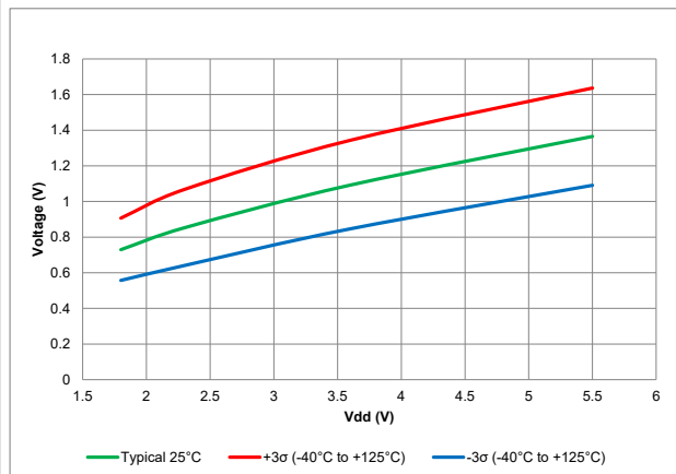
Figure 40-56. Input Level TTL
