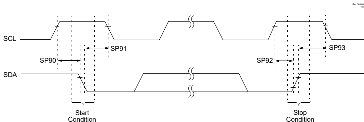
Figure 39-20. I 2 C Bus Start/Stop Bits Timing
