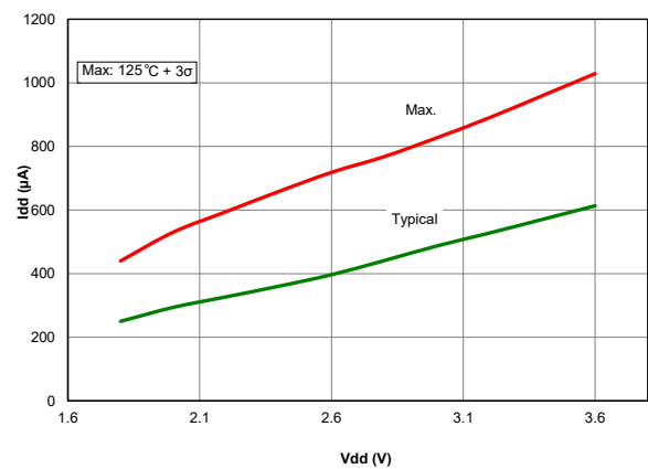
Figure 40-50. I_{DD} , ECM Oscillator, F_{OSC} = 4MHz , PIC18LF67K40 only
