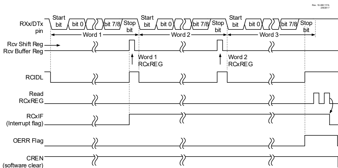
Figure 28-5. Asynchronous Reception
