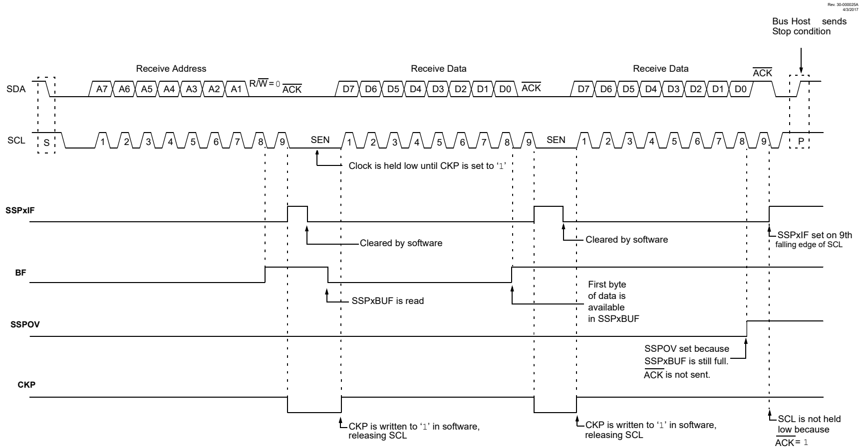
Figure 27-15. I 2 C Client, 7-Bit Address, Reception (SEN = 1, AHEN = 0, DHEN = 0)
