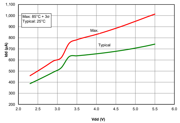
Figure 40-44. I_{DD} , ECM Oscillator, F_{OSC} = 4\text{MHz} , PIC18F67K40 only
