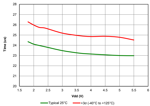
Figure 40-102. Wake From Sleep, V_{REGPM} = 0 , HFINTOSC = 16MHz
