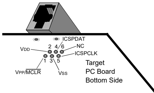
Figure 36-1. ICD RJ-11 Style Connector Interface
