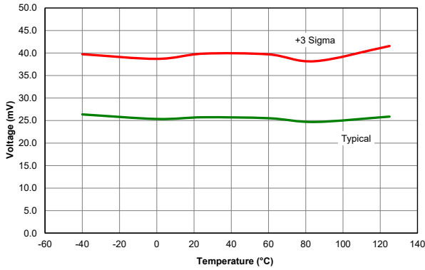
Figure 40-20. Brown-Out Reset Hysteresis, Trip Point (BORV = 11) for PIC18LF67K40 only
