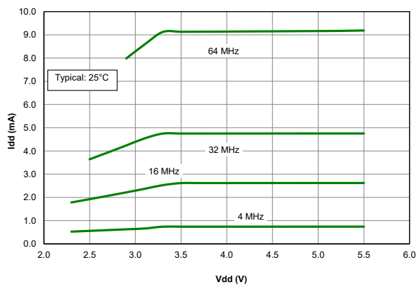
Figure 40-47. I_{DD} , HFINTOSC, Typical, PIC18F67K40 only
