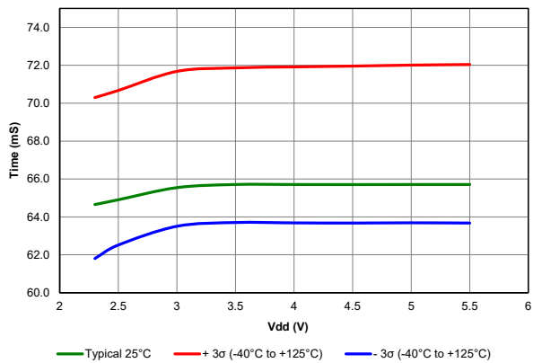
Figure 40-83. Power-up Timer Period, PIC18F67K40 only
