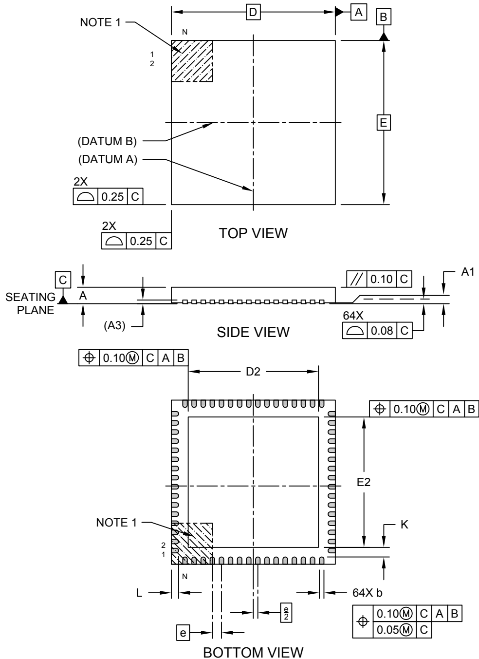
Microchip Technology Drawing C04-149 [MR] Rev E Sheet 1 of 2
