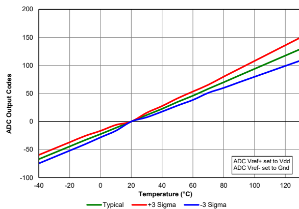
Figure 40-93. Temperature Indicator, Slope Normalized to 20°C, Low Range, V_{DD} = 2.3V , PIC18LF67K40 only
