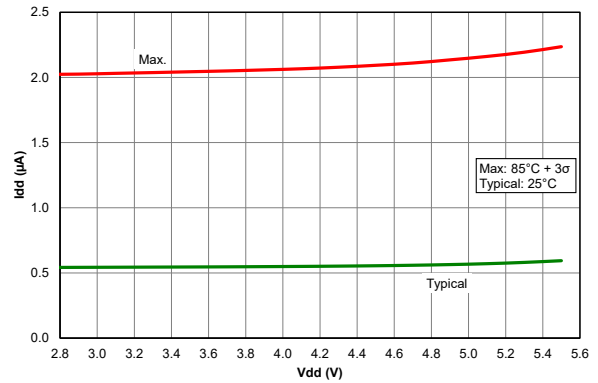
Figure 40-68. I_{PD} , Low-power Brown-out Reset, LPBOR = 0, PIC18F67K40 only
