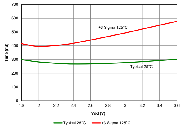
Figure 40-24. Comparator Response Time, Rising Edge, PIC18LF67K40 only
