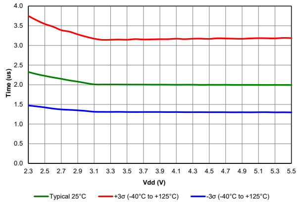
Figure 40-10. ADC RC Oscillator Period, PIC18F67K40 only
