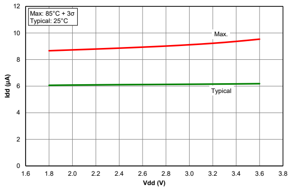
Figure 40-69. I_{PD} , Comparator, PIC18LF67K40 only
