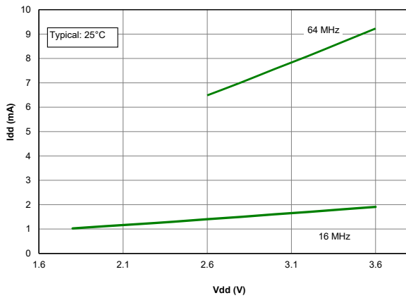
Figure 40-51. I_{DD} , ECH Oscillator, Typical, PIC18LF67K40 only
