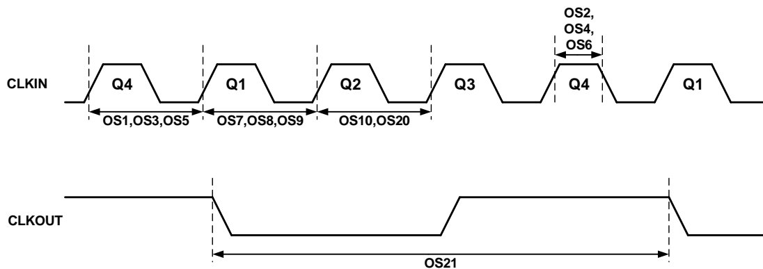
Figure 39-5. Clock Timing
