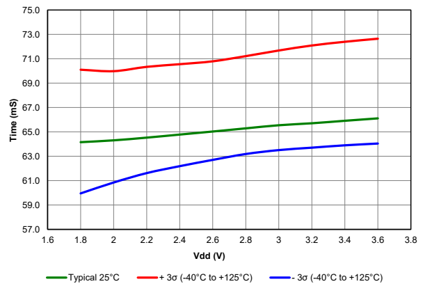
Figure 40-84. Power-up Timer Period, PIC18LF67K40 only
