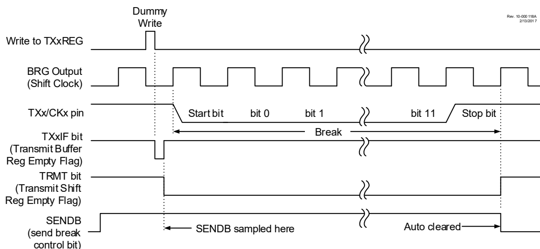
Figure 28-9. Send Break Character Sequence
