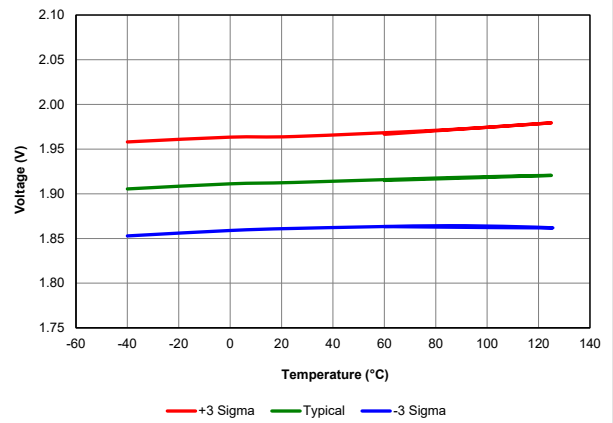
Figure 40-19. Brown-Out Reset Voltage, Trip Point (BORV = 11) for PIC18LF67K40 only
