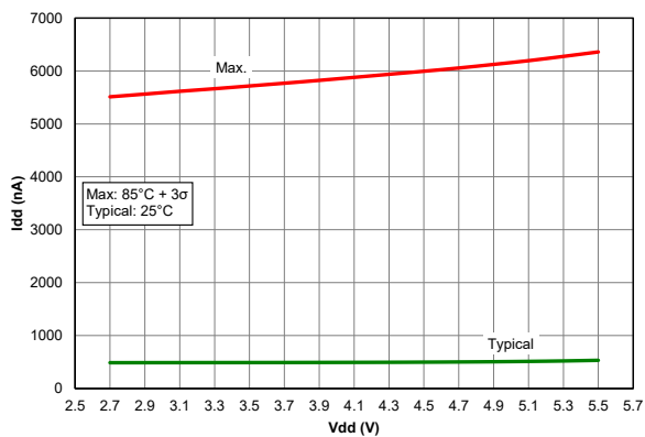
Figure 40-75. I_{PD} Base, VREGPM = 11, PIC18F67K40 only
