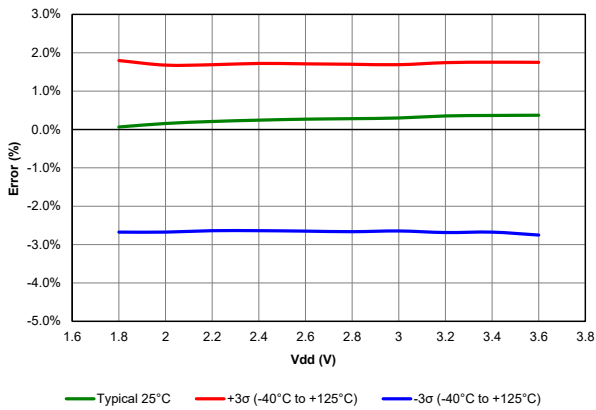
Figure 40-39. HFINTOSC Typical Frequency Error, PIC18LF67K40 only
