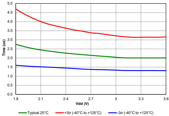
Figure 40-9. ADC RC Oscillator Period, PIC18LF67K40 only
