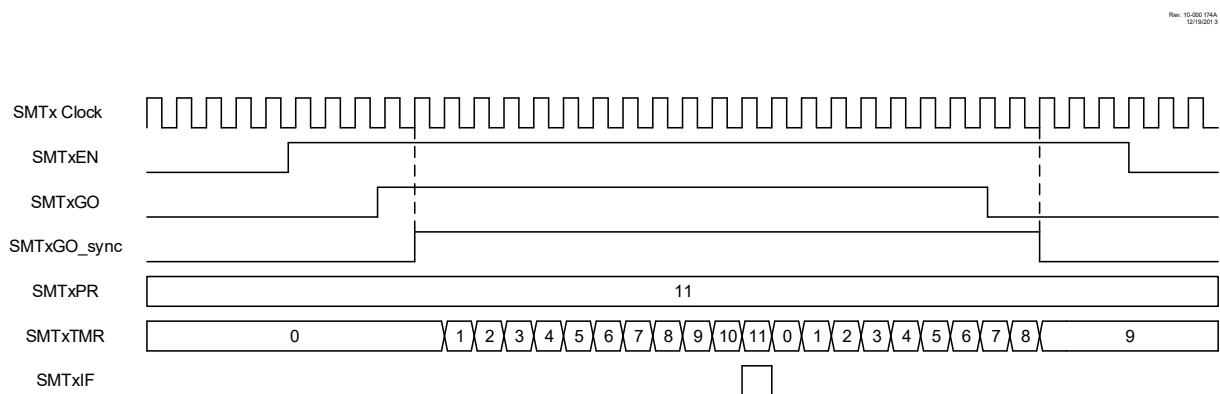
Figure 25-2. Timer Mode Timing Diagram
