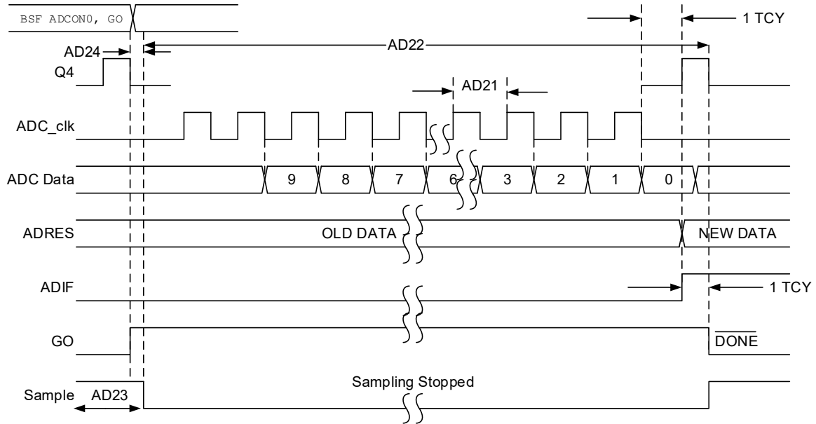
Figure 39-10. ADC Conversion Timing (ADC Clock F_{OSC} -Based)
