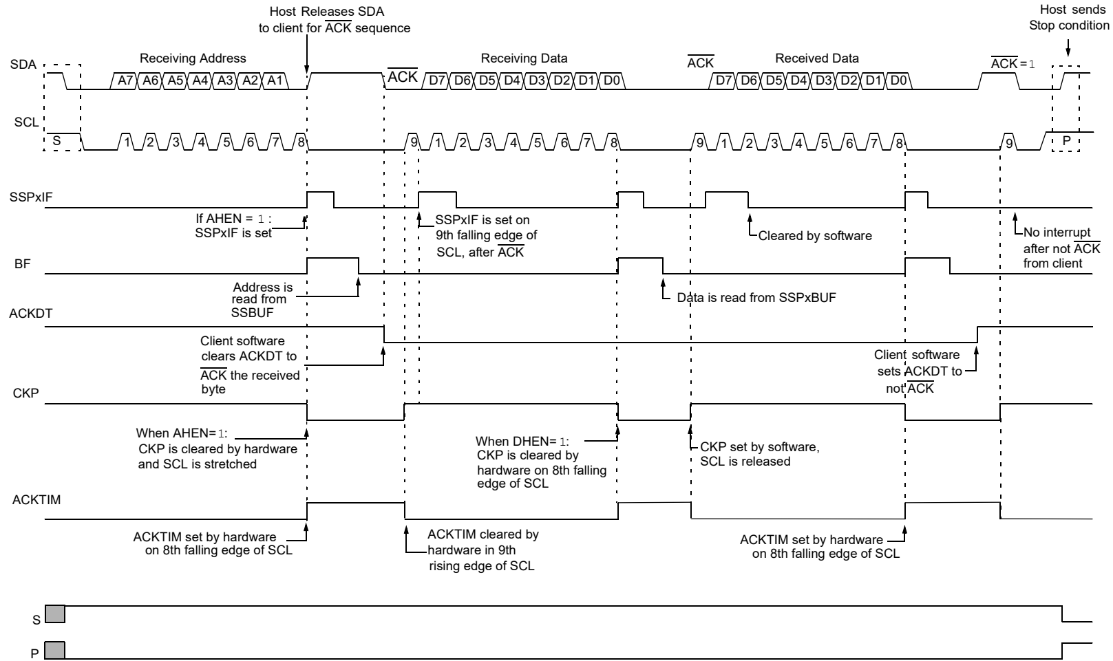
Figure 27-16. I 2 C Client, 7-Bit Address, Reception (SEN = 0, AHEN = 1, DHEN = 1)
