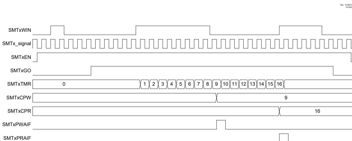
Figure 25-21. Windowed Counter Mode, Single Acquisition Timing Diagram
