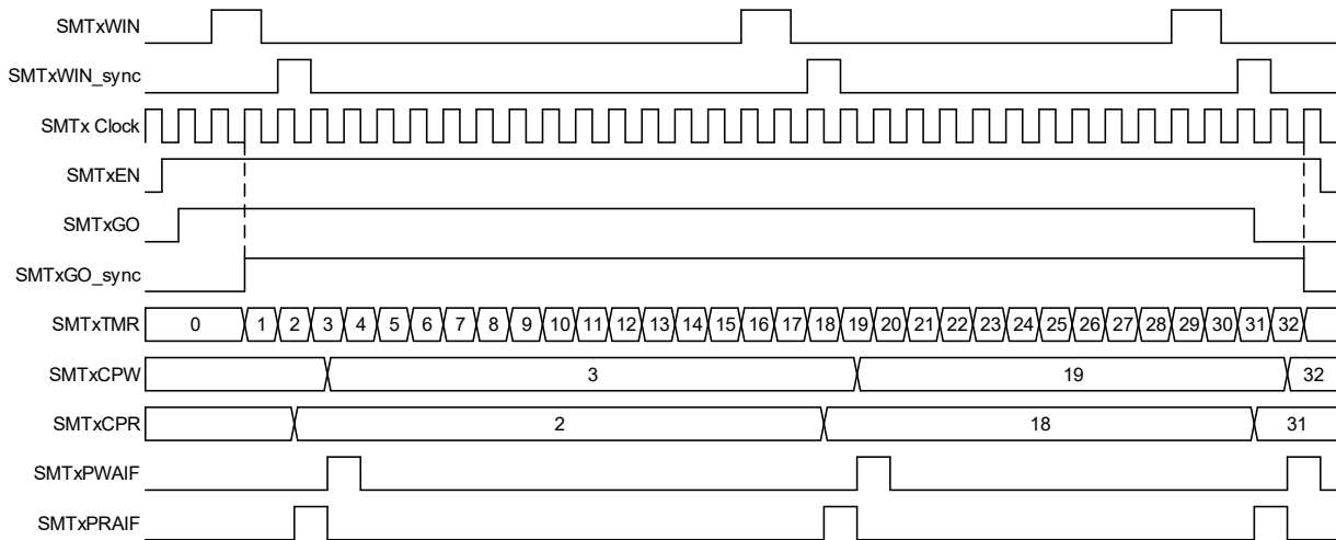
Figure 25-16. Capture Mode, Single Acquisition Timing Diagram
