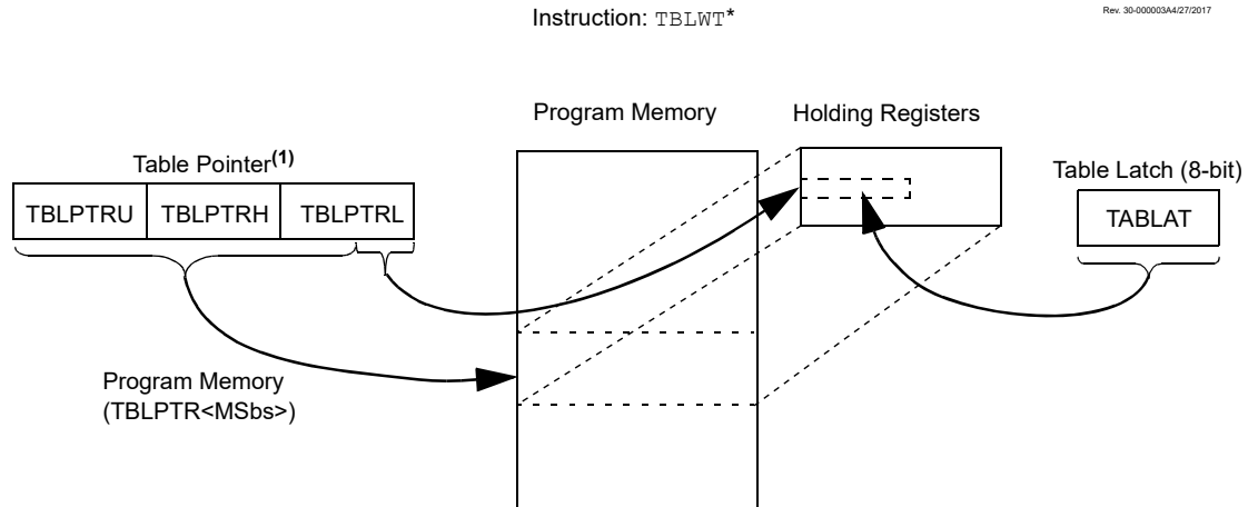
Figure 11-2. Table Write Operation
