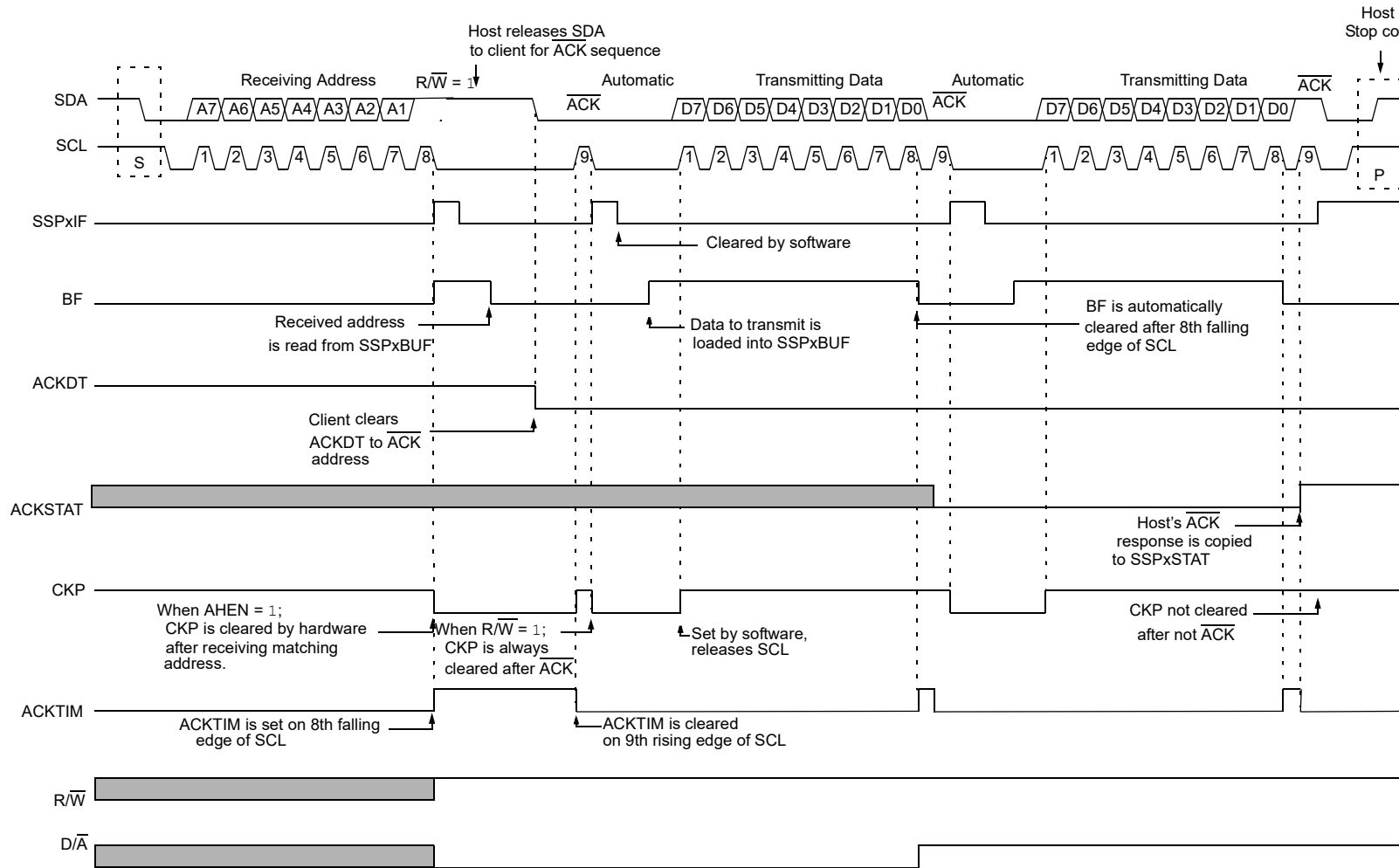
Figure 27-19. I 2 C Client, 7-Bit Address, Transmission (AHEN = 1)
