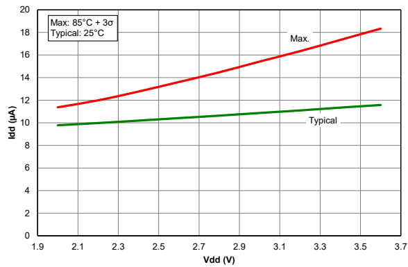
Figure 40-65. I_{PD} , Brown-out Reset, BORV = 1, PIC18LF67K40 only
