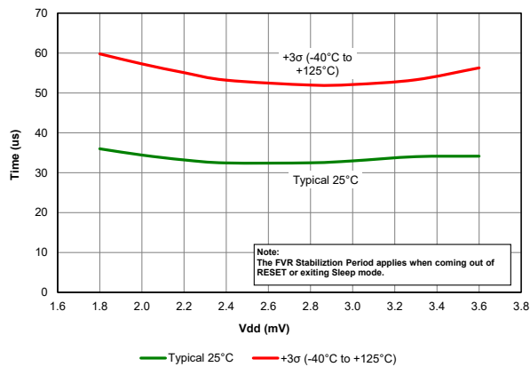
Figure 40-33. FVR Stabilization Period, PIC18LF67K40 only
