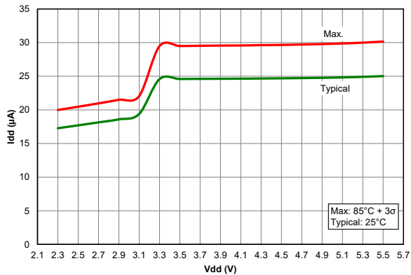
Figure 40-73. I_{PD} Base, VREGPM = 01, PIC18F67K40 only
