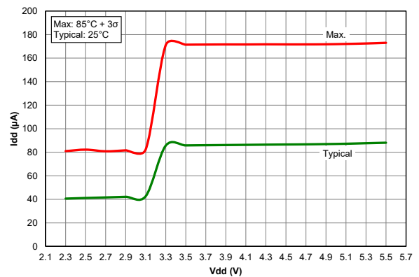
Figure 40-72. I_{PD} Base, VREGPM = 00, PIC18F67K40 only
