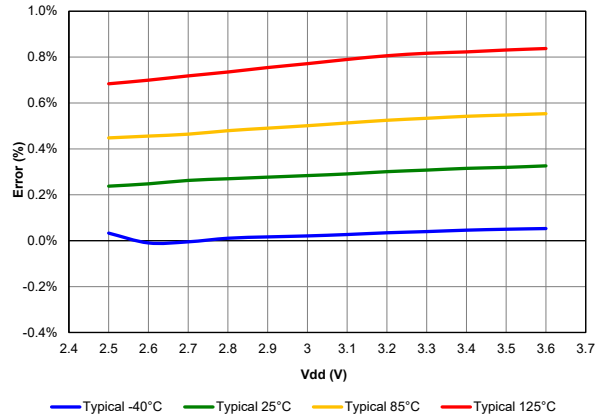
Figure 40-36. Typical FVR Voltage Error 2x, PIC18LF67K40 only
