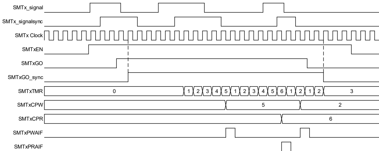
Figure 25-8. High and Low Measurement Mode, Single Acquisition Timing Diagram
