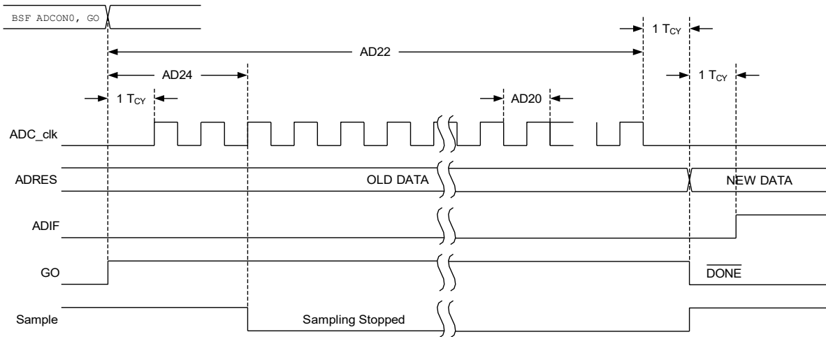
Figure 39-11. ADC Conversion Timing (ADC Clock from F_{RC} )
