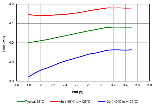
Figure 40-107. Watchdog Timer Time-out Period, PIC18LF67K40 only
