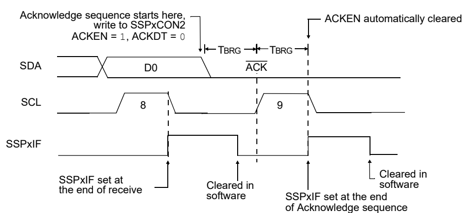
Figure 27-30. Acknowledge Sequence Waveform
