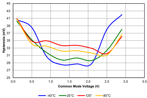
Figure 40-29. Comparator Hysteresis, V_{DD} = 3.0V , PIC18LF67K40 only
