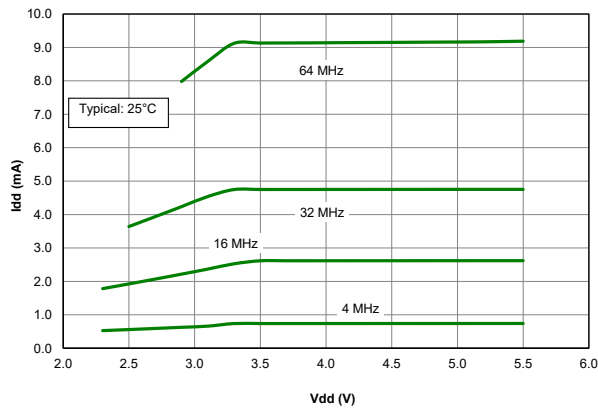
Figure 40-47. I_{DD} , HFINTOSC, Typical, PIC18F67K40 only
