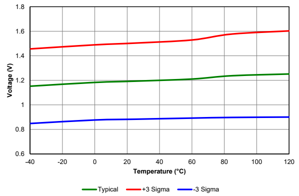
Figure 40-82. POR Rearm Voltage, Normal Power Mode, PIC18LF67K40 only
