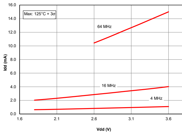
Figure 40-49. I_{DD} , HFINTOSC, Maximum, PIC18LF67K40 only
