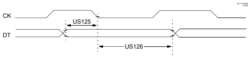
Figure 39-15. EUSART Synchronous Receive (Host/Client) Timing
