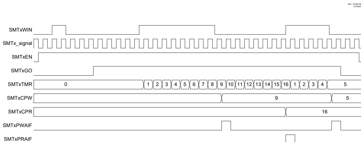
Figure 25-20. Windowed Counter Mode, Repeat Acquisition Timing Diagram
