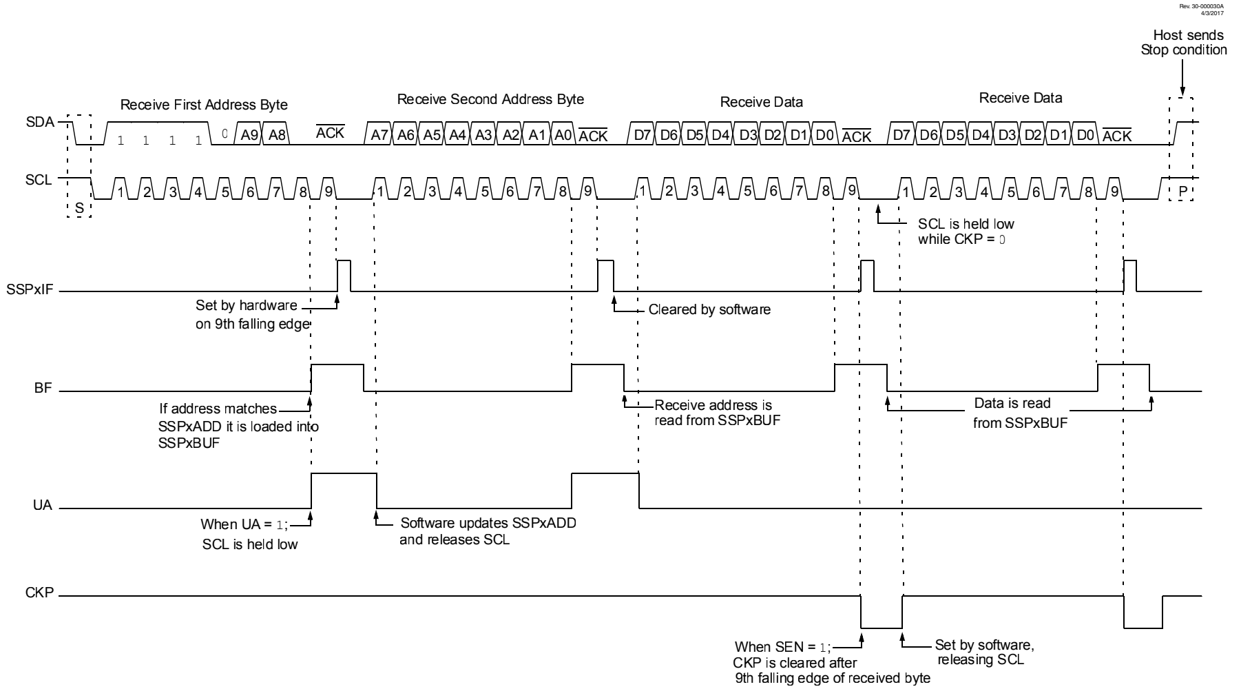
Figure 27-20. I 2 C Client, 10-Bit Address, Reception (SEN = 1, AHEN = 0, DHEN = 0)
