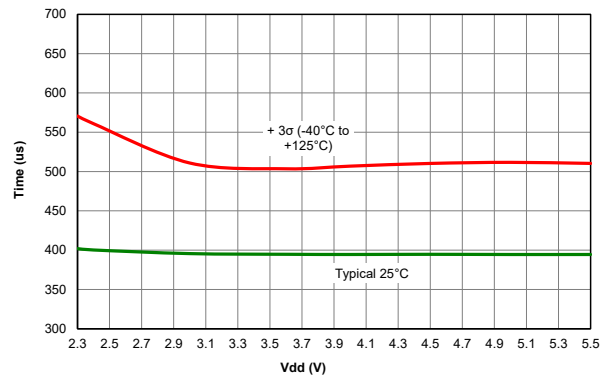
Figure 40-104. Wake From Sleep, VREGPM = 1, LFINTOSC, PIC18F67K40 only
