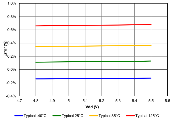
Figure 40-38. Typical FVR Voltage Error 4x, PIC18F67K40 only
