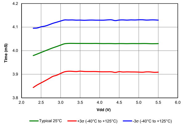
Figure 40-106. Watchdog Timer Time-out Period, PIC18F67K40 only
