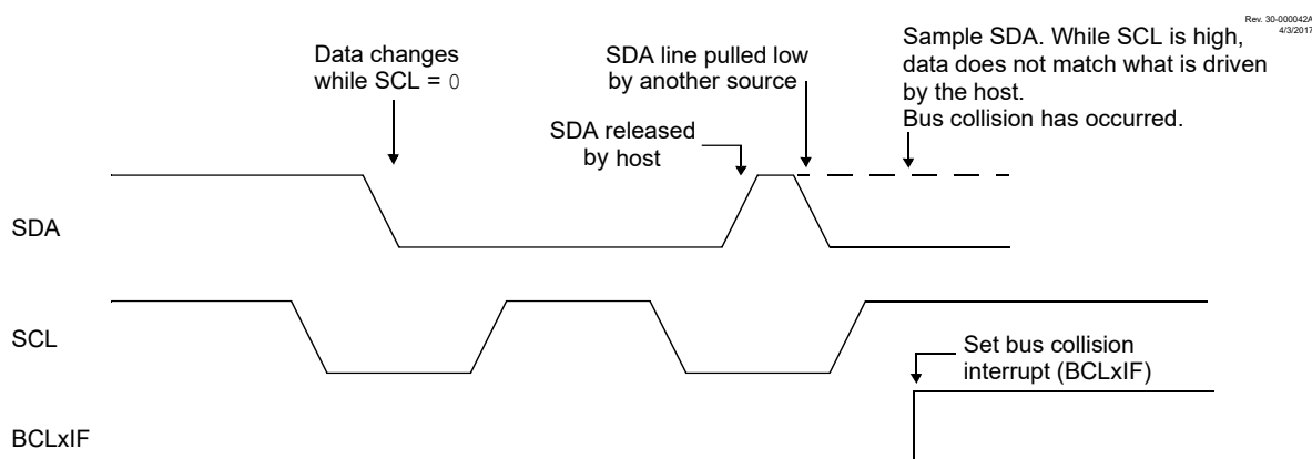
Figure 27-32. Bus Collision Timing for Transmit and Acknowledge
