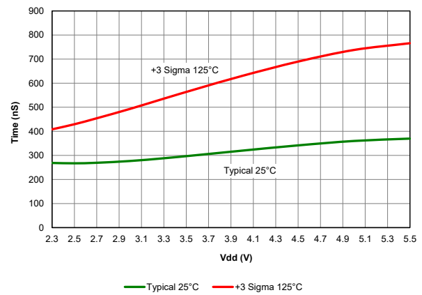
Figure 40-26. Comparator Response Time, Rising Edge, PIC18F67K40 only
