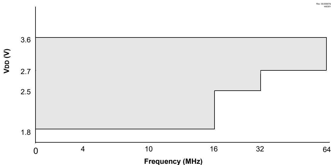
Figure 39-2. Voltage Frequency Graph, -40^{\circ}\text{C} \leq T_A \leq +125^{\circ}\text{C} , for PIC18LF67K40 Devices only
