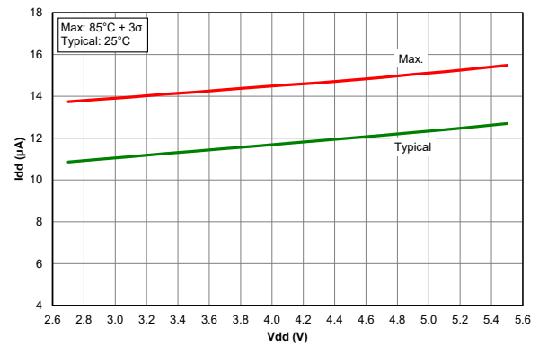
Figure 40-66. I_{PD} , Brown-out Reset, BORV = 1, PIC18F67K40 only
