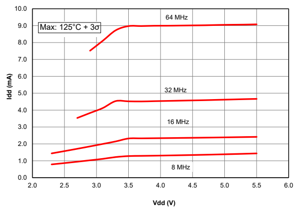
Figure 40-46. I_{DD} , ECH Oscillator, Maximum, PIC18F67K40 only
