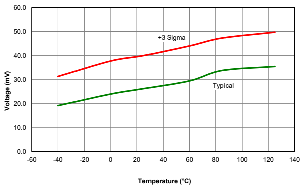
Figure 40-18. LPBOR Reset Hysteresis, PIC18LF67K40 only
