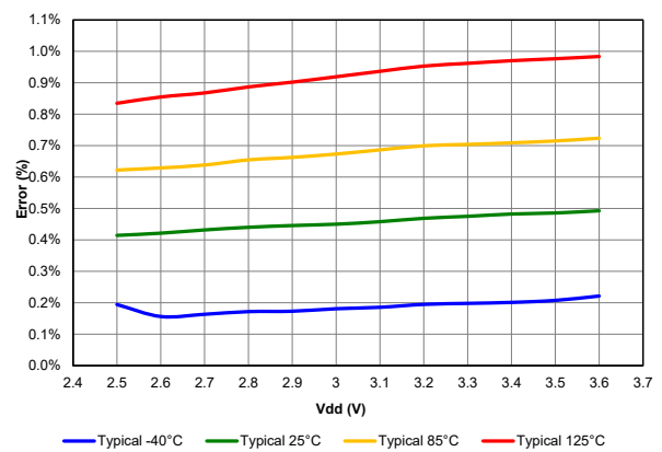
Figure 40-34. Typical FVR Voltage Error 1x, PIC18LF67K40 only
