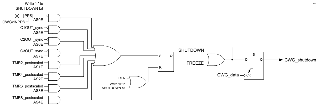
Figure 24-14. CWG Shutdown Block Diagram
