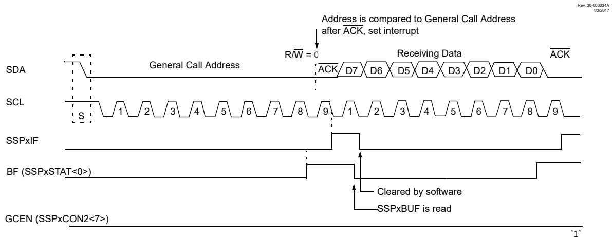
Figure 27-24. Client Mode General Call Address Sequence
