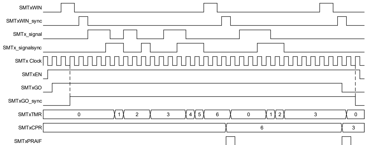
Figure 25-12. Gated Windowed Measurement Mode, Single Acquisition Timing Diagram
