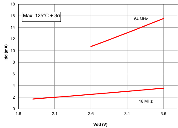
Figure 40-52. I_{DD} , ECH Oscillator, Maximum, PIC18LF67K40 only
