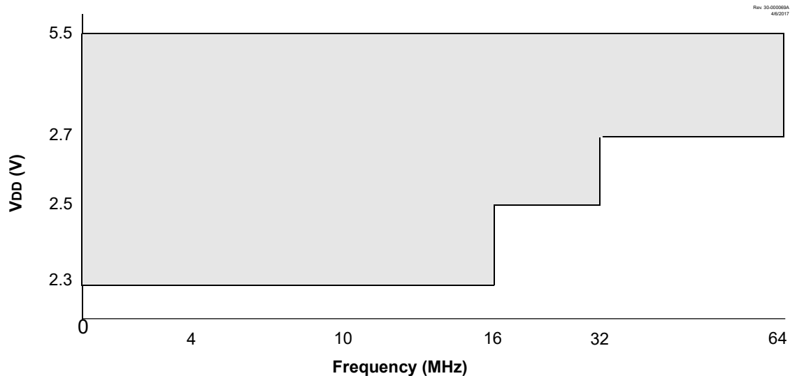
Figure 39-1. Voltage Frequency Graph, -40°C ≤ T A ≤ +125°C, for PIC18F67K40 only
