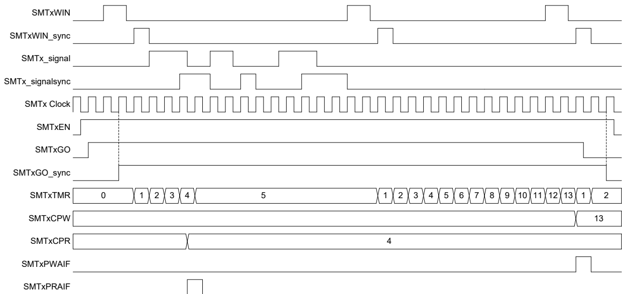
Figure 25-14. Time of Flight Mode, Single Acquisition Timing Diagram
