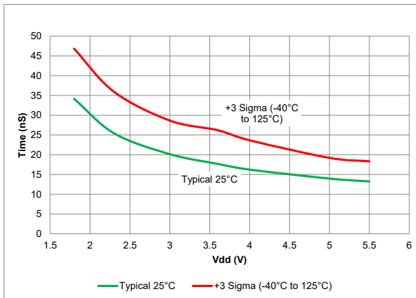
Figure 40-57. I/O Rise Time, Slew Rate Control Enabled
