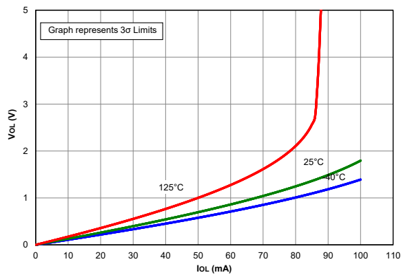
Figure 40-95. V_{OL} vs I_{OL} , Over Temperature, V_{DD} = 5.0V , PIC18F67K40 only
