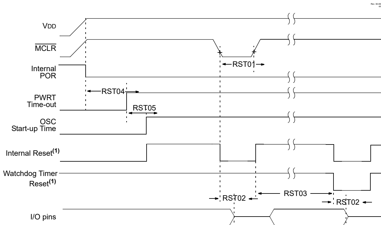
Figure 39-8. Reset, Watchdog Timer, Oscillator Start-up Time and Power-up Timer Timing
