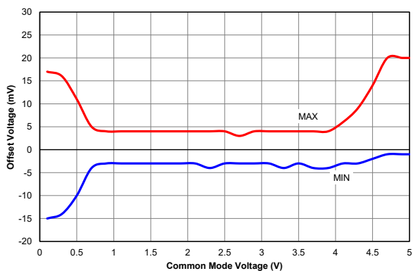
Figure 40-31. Comparator Offset, V_{DD} = 5.0V , 25°C, PIC18F67K40 only
