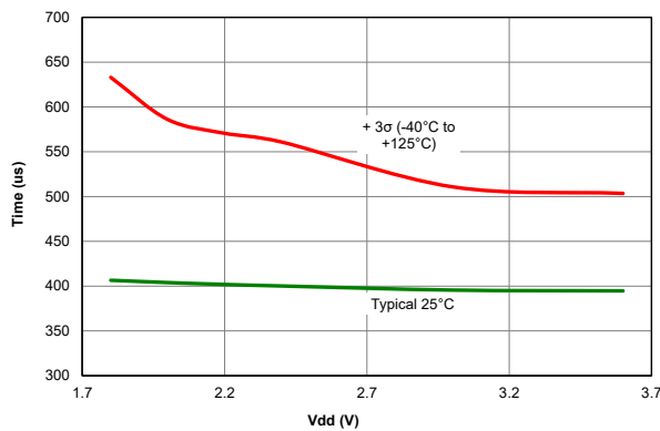
Figure 40-105. Wake From Sleep, LFINTOSC, PIC18LF67K40 only
