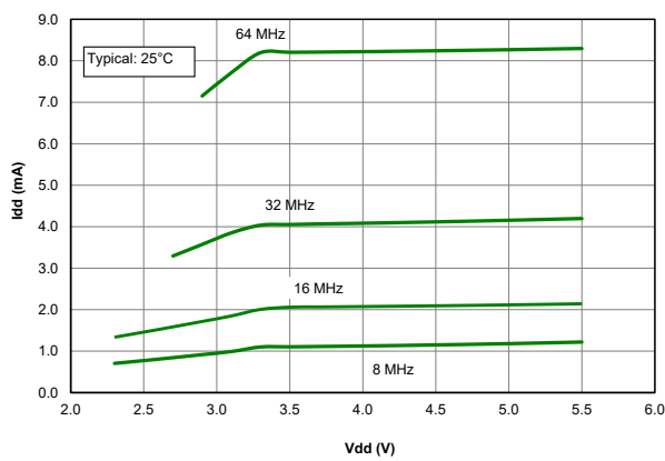
Figure 40-45. I_{DD} , ECH Oscillator, Typical, PIC18F67K40 only
