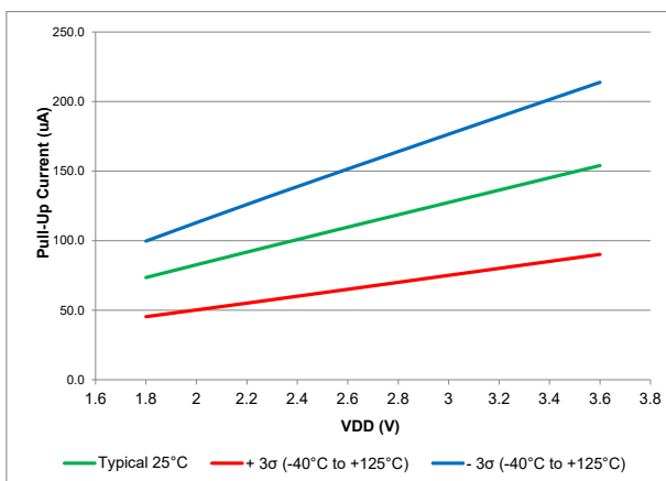
Figure 40-109. Weak Pull-up Current, PIC18LF67K40 only
