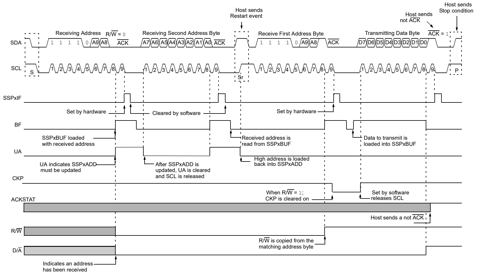
Figure 27-22. I 2 C Client, 10-Bit Address, Transmission (SEN = 0, AHEN = 0, DHEN = 0)
