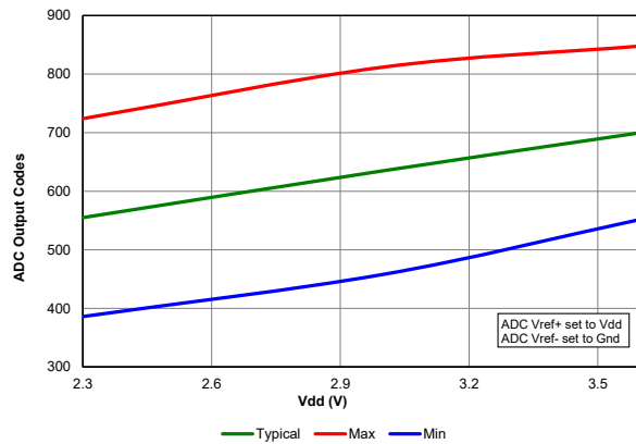
Figure 40-87. Temperature Indicator, Initial Offset, Low Range, Temp = 20°C, PIC18LF67K40 only
