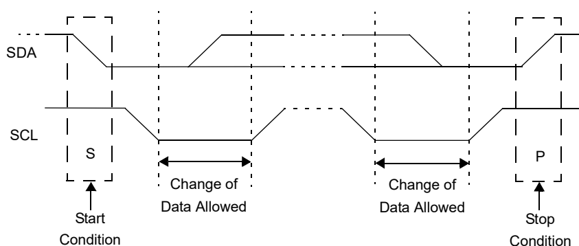
Figure 27-12. I 2 C Start and Stop Conditions
