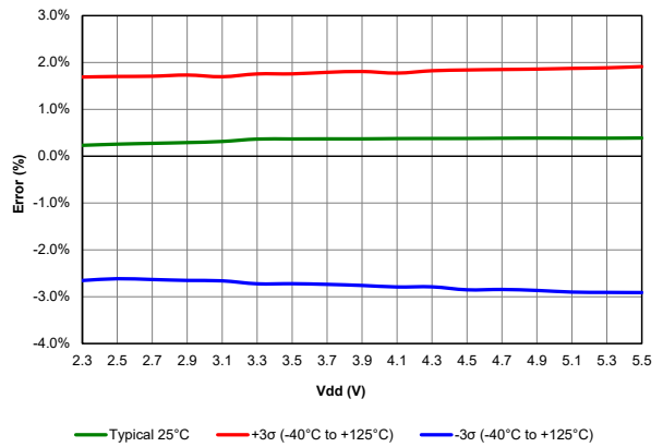
Figure 40-40. HFINTOSC Typical Frequency Error, PIC18F67K40 only
