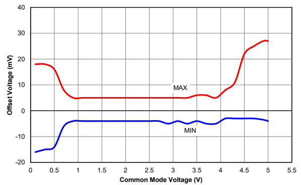
Figure 40-32. Comparator Offset, V_{DD} = 5.5V , from -40^{\circ}C to 125^{\circ}C , PIC18F67K40 only
