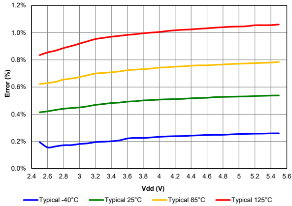
Figure 40-35. Typical FVR Voltage Error 1x, PIC18F67K40 only
