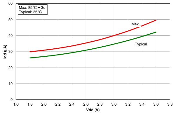
Figure 40-63. I_{PD} , Fixed Voltage Reference (FVR), PIC18LF67K40 only
