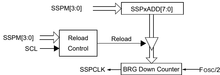
Figure 28-40. Baud Rate Generator Block Diagram
