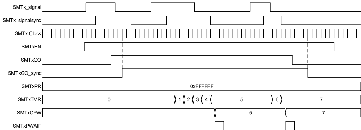
Figure 25-4. Gated Timer Mode, Single Acquisition Timing Diagram
