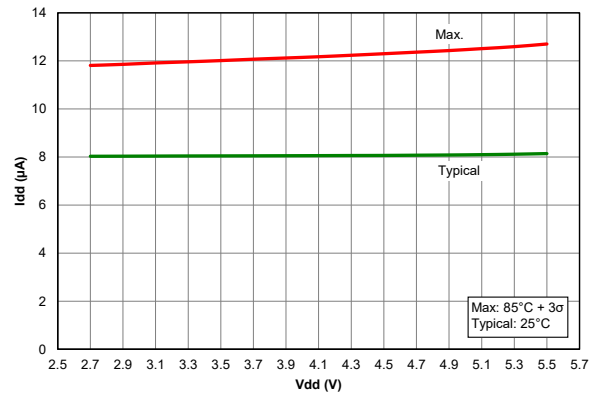
Figure 40-74. I_{PD} Base, VREGPM = 10, PIC18F67K40 only
