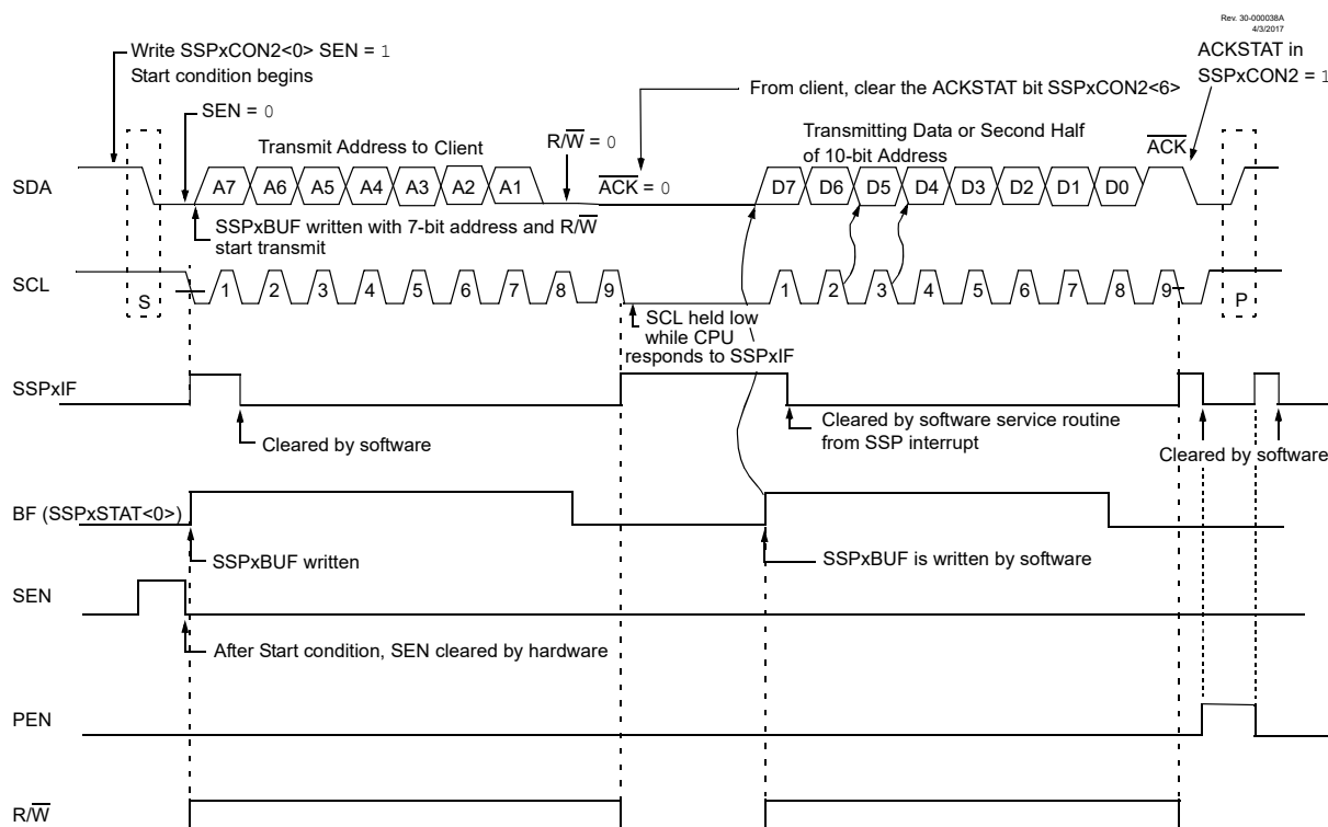
Figure 27-28. I 2 C Host Mode Waveform (Transmission, 7- or 10-Bit Address)
