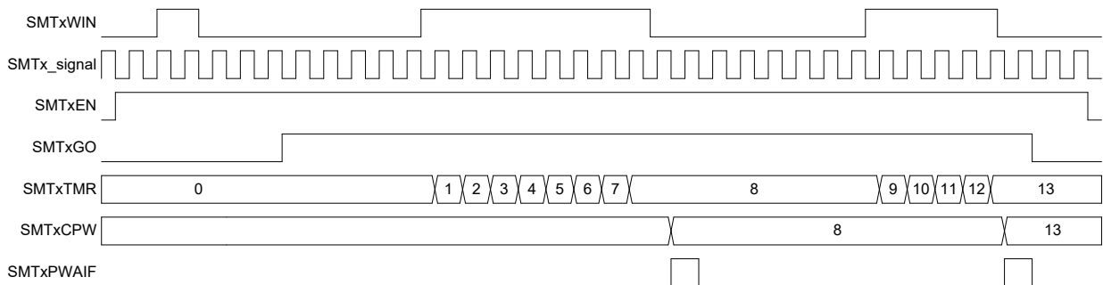
Figure 25-19. Gated Counter Mode, Single Acquisition Timing Diagram
