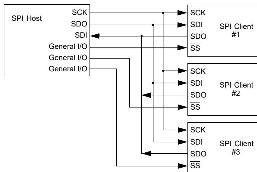
Figure 27-2. SPI Host and Multiple Client Connection
