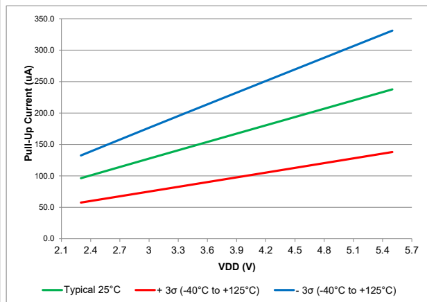
Figure 40-108. Weak Pull-up Current, PIC18F67K40 only
