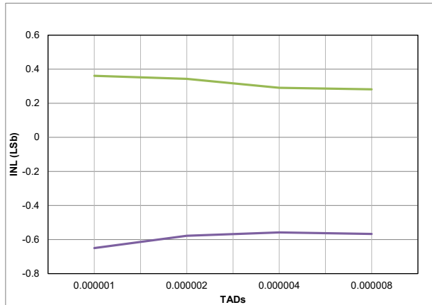
Figure 40-5. ADC, Single-Ended INL, V_{DD} = 3.0V , V_{REF} = 3.0V
