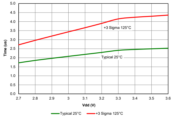
Figure 40-21. BOR Response Time, PIC18LF67K40 only
