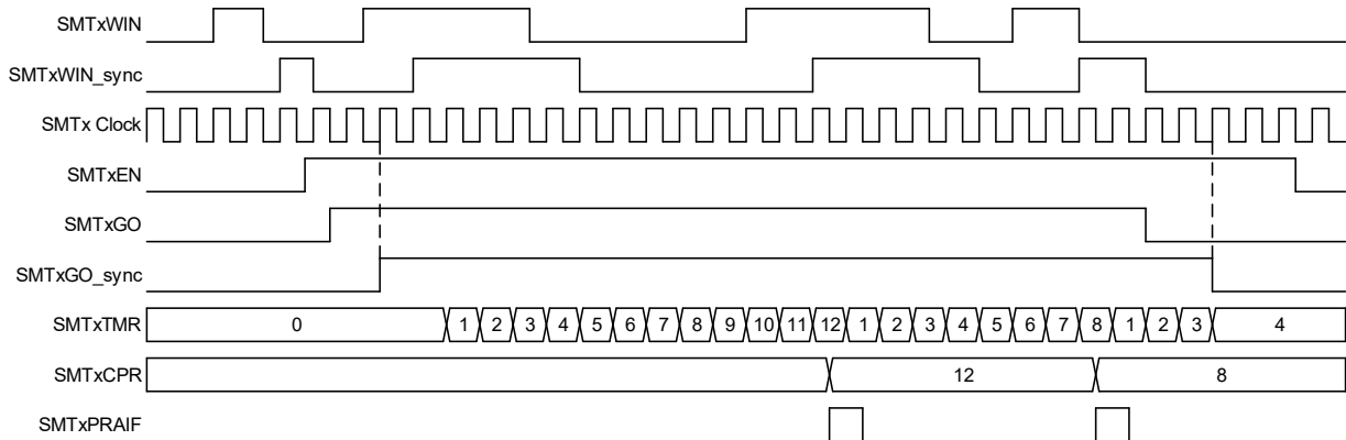
Figure 25-10. Windowed Measurement Mode, Single Acquisition Timing Diagram
