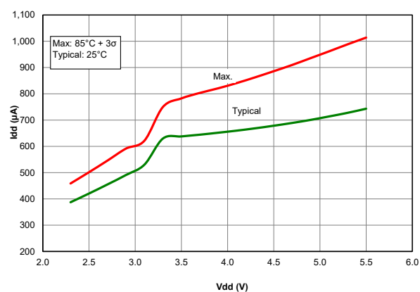
Figure 40-44. I_{DD} , ECM Oscillator, F_{OSC} = 4\text{ MHz} , PIC18F67K40 only
