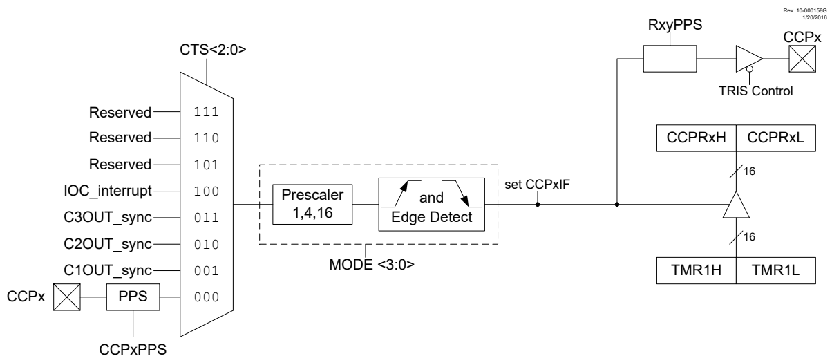
Figure 21-1. Capture Mode Operation Block Diagram
