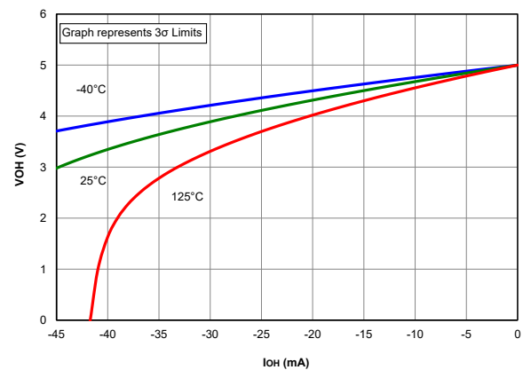
Figure 40-94. V_{OH} vs I_{OH} , Over Temperature, V_{DD} = 5.0V , PIC18F67K40 only
