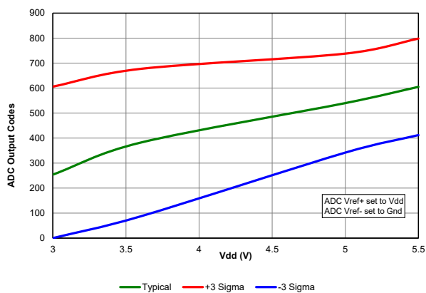
Figure 40-85. Temperature Indicator, Initial Offset, High Range, Temp = 20°C, PIC18F67K40 only
