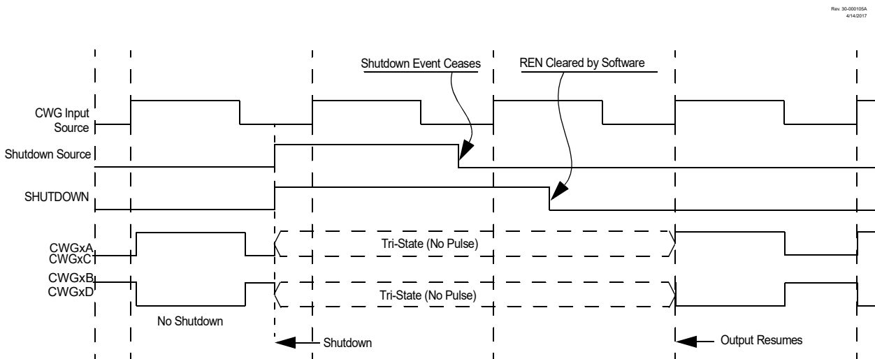
Figure 24-15. Shutdown Functionality, Auto-Restart Disabled ( REN = 0 , LSAC = 01 , LSBD = 01 )
