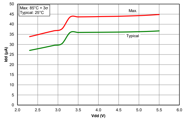
Figure 40-70. I_{PD} , Comparator, PIC18F67K40 only
