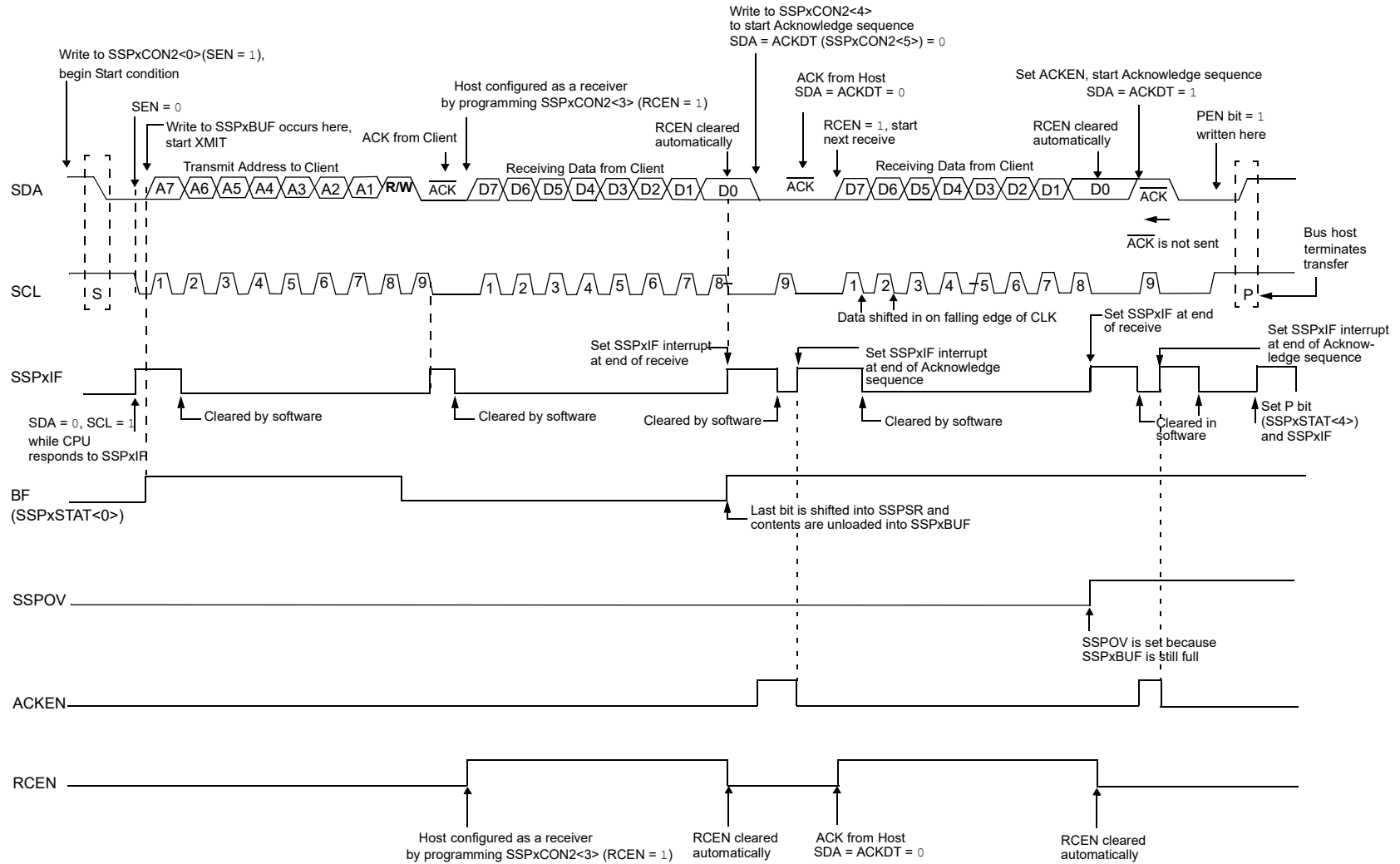
Figure 27-29. I 2 C Host Mode Waveform (Reception, 7-Bit Address)
