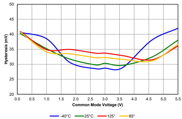
Figure 40-30. Comparator Hysteresis, V_{DD} = 5.5V , PIC18F67K40 only
