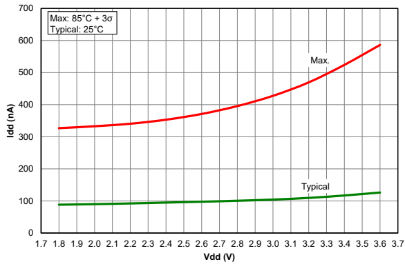
Figure 40-67. I_{PD} , Low-power Brown-out Reset, LPBOR = 0, PIC18LF67K40 only
