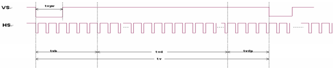
Fig2. Vertical input timing diagram
