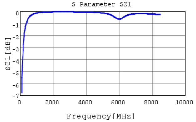
GCM1555C1H8R2DA16 S21 DCOV, 25degC
