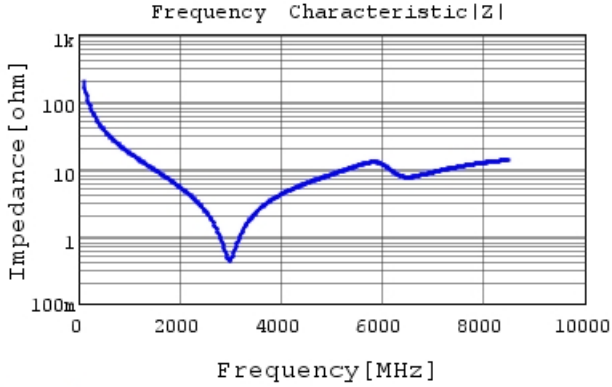
GCM1555C1H8R2DA16 |Z| DCOV, 25degC
