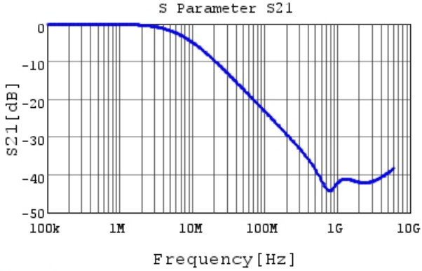
NFM18CC102R1C3 S21 DCOV,25degC, Feedthrough
