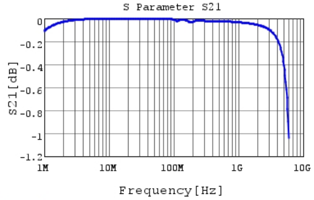
GRM3195C1H103JA01 S21 DCOV, 25degC
