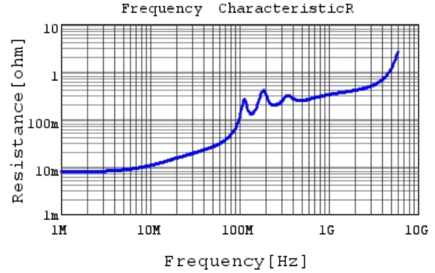
GRM3195C1H103JA01 R DCOV, 25degC
