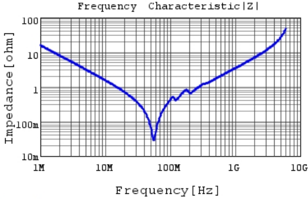
GRM3195C1H103JA01 |Z| DCOV, 25degC
