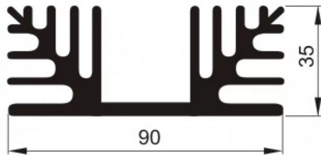
Technical Drawing
