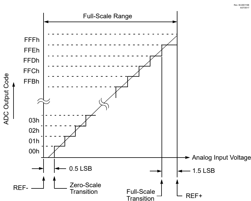
Figure 33-10. ADC Transfer Function
