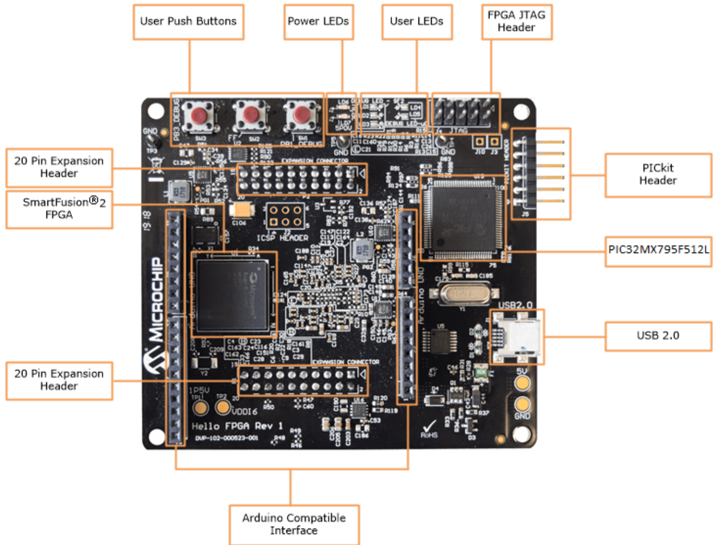
Figure 1. Hello FPGA Kit
