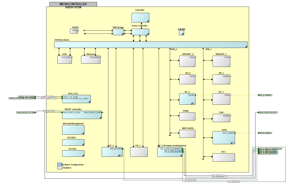
Figure 1-6. MSS Component Configuration
