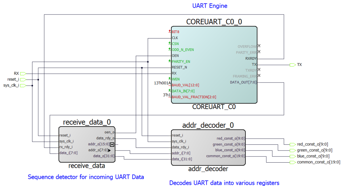
Figure 1-7. UART_interface
