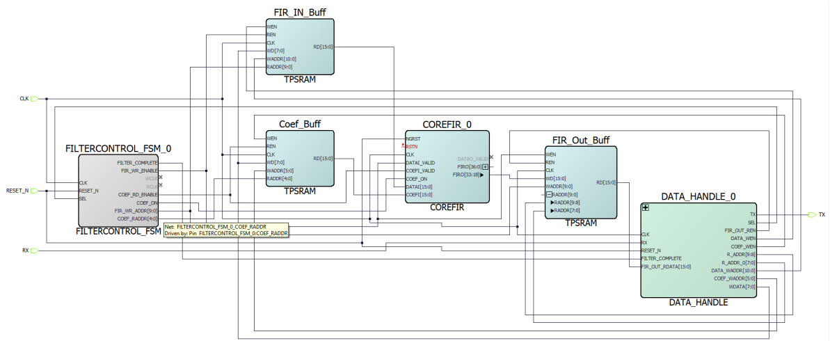
Figure 3-4. FIR_FILTER Module
