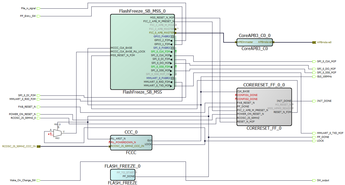
Figure 3-3. FlashFreeze_SB_0 Module
