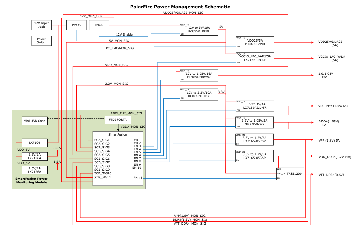
Figure 10 • Power Management
