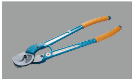
1530 電纜剪 CABLE CUTTERS RYC-60 適用電纜:最大60sq / AWG 1/0 / DIN 50mm 2 RYC-100 適用電纜:最大100sq / AWG 4/0 / DIN 120mm 2 RYC-250 適用電纜:最大250sq / AWG 500mcm / DIN 260mm 2 RYC-400 適用電纜:最大400sq / AWG 600mcm / DIN 300mm 2 RYC-500 適用電纜:最大500sq
