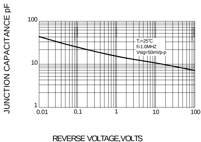
FIG.5-TYPICAL JUNCTION CAPACITANCE
