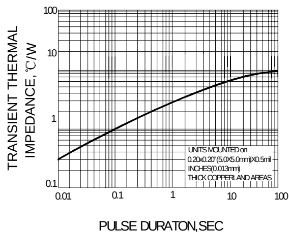
FIG.6-TRANSIENT THERMAL IMPEDANCE
