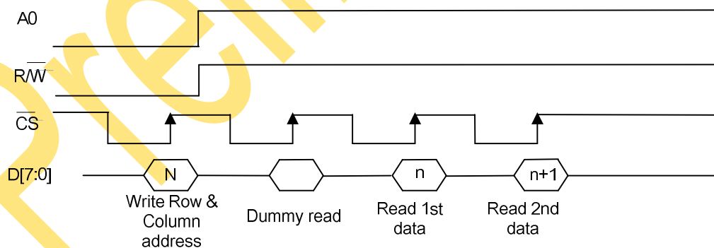
Figure 5 Read RAM data process—insertion of dummy read
