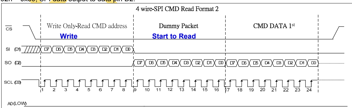
Figure 12 4-wire SPI Read Only-Read CMD data
