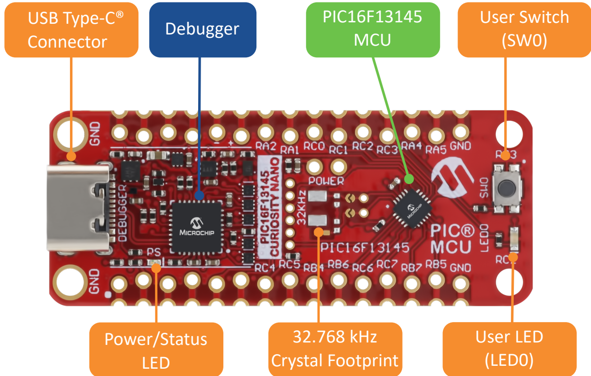
Figure 1-1. PIC16F13145 Curiosity Nano Board Overview
