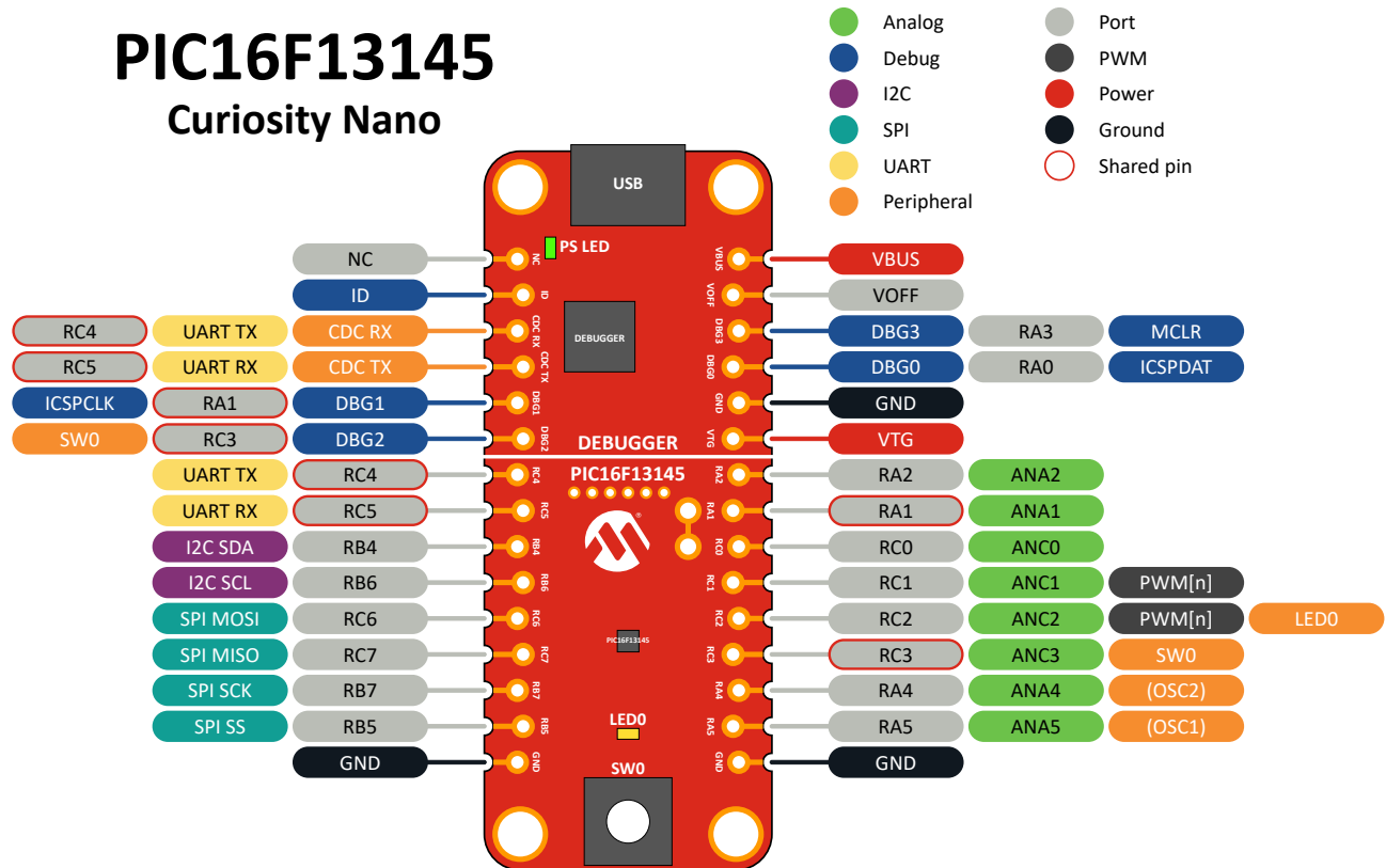
Figure 1-3. PIC16F13145 Curiosity Nano Pinout
