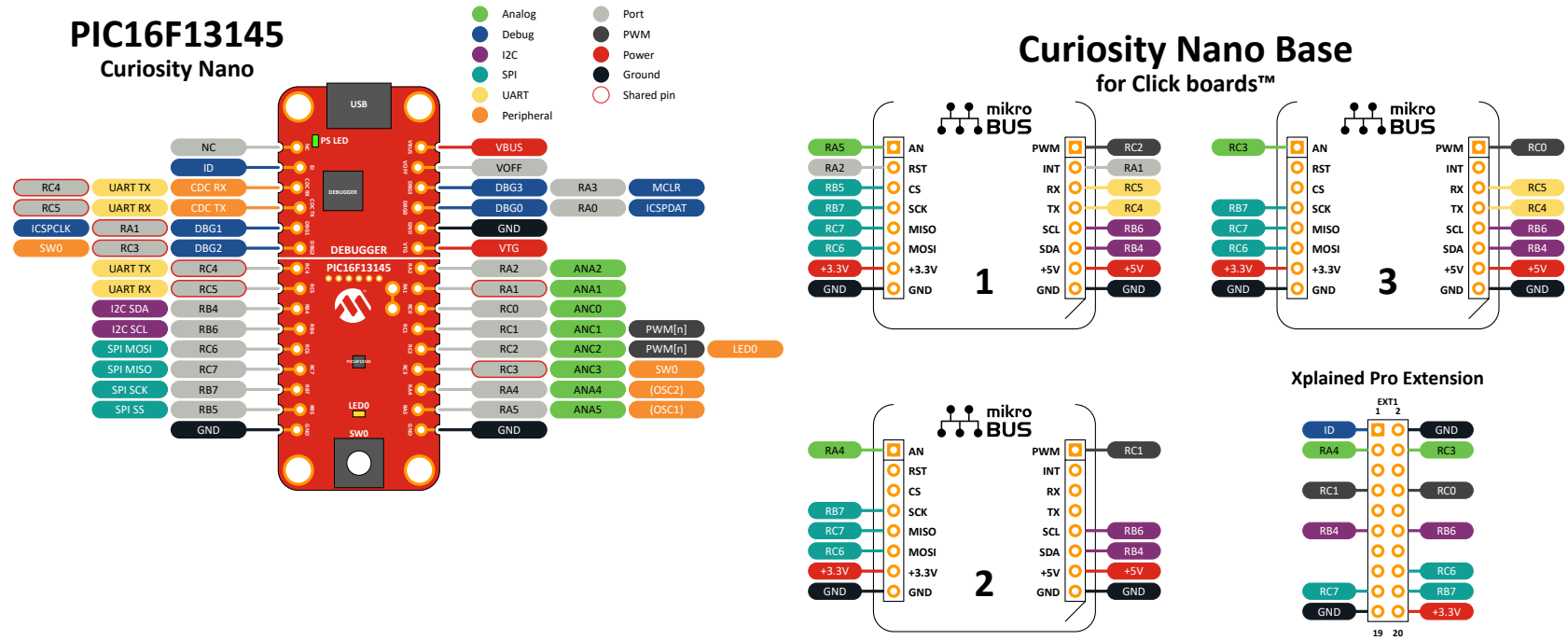
Figure 6-5. PIC16F13145 Curiosity Nano Pinout Mapping
