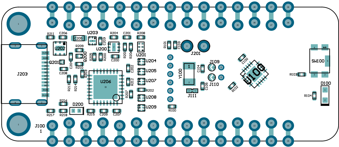
Figure 6-3. PIC16F13145 Curiosity Nano Assembly Drawing Top
