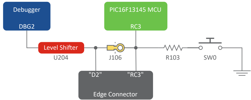
Figure 4-4. PIC16F13145 Curiosity Nano SW0 Block Diagram
