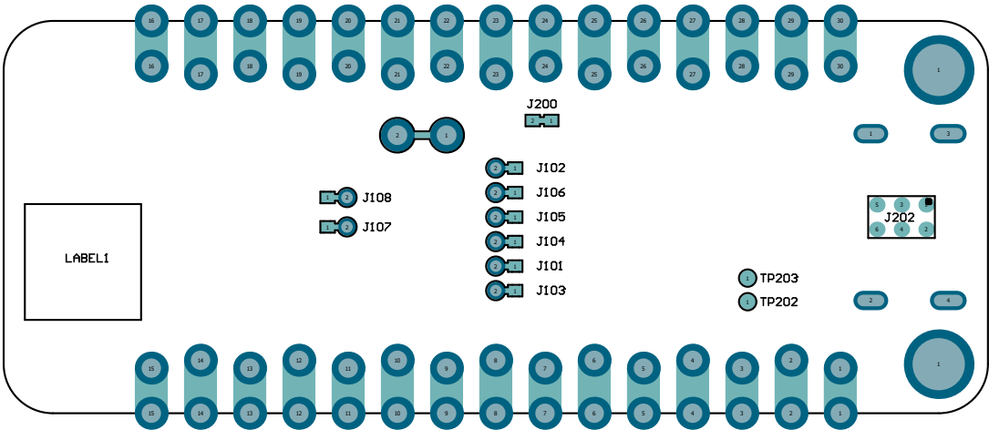
Figure 6-4. PIC16F13145 Curiosity Nano Assembly Drawing Bottom
