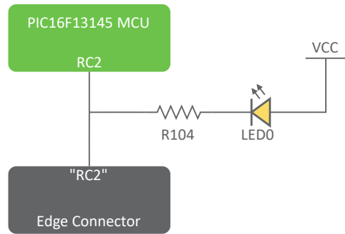
Figure 4-3. PIC16F13145 Curiosity Nano LED0 Block Diagram
