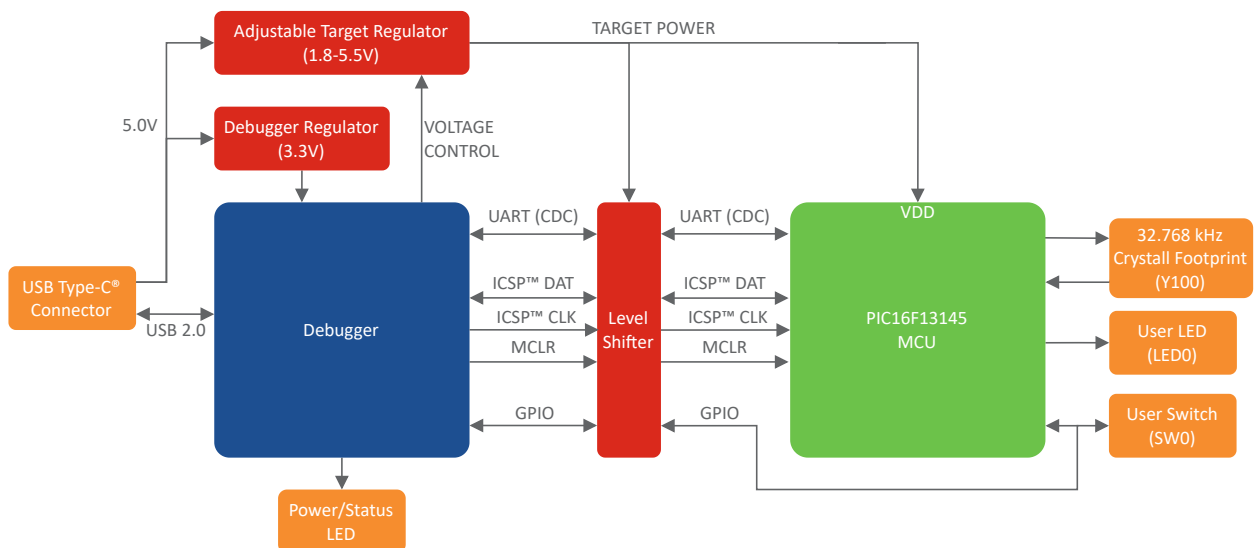
Figure 1-2. PIC16F13145 Curiosity Nano Board Block Diagram
