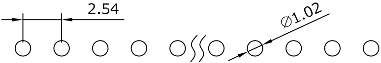
Recommended PCB Layout (PCB TOLERANCE ±0.05)
