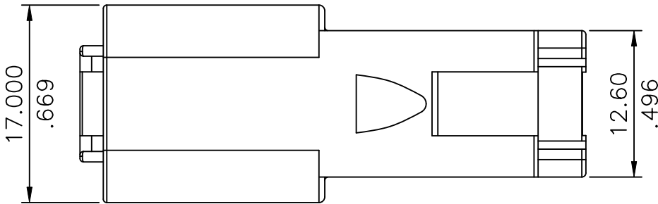
HOUSING
