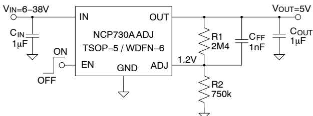
Figure 2. Adjustable Output Voltage Application (No PG)
