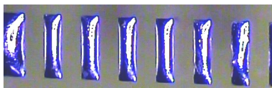
Solder balling with PacIFic 2009MLF
