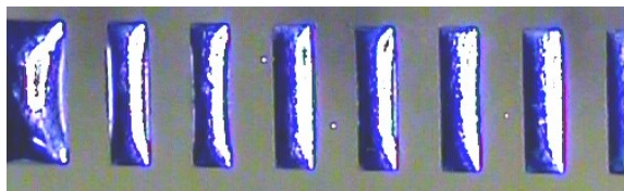
Solder balling with a conventional VOC-free flux
