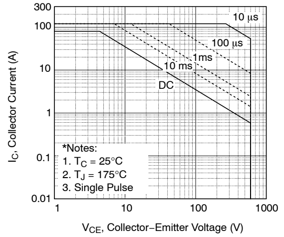
Figure 16. SOA Characteristics
