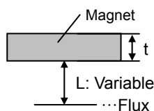
Fig.40 Magnet Dimensions and Flux Density Measuring Point
