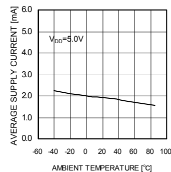
Fig.26 I_{DD} - Ambient temperature
