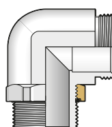
Winkel Elbow
