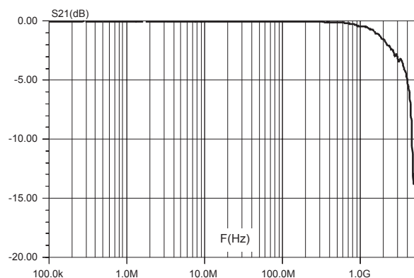
Figure 4. Frequency response
