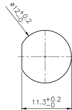
PANEL CUT-OUT
