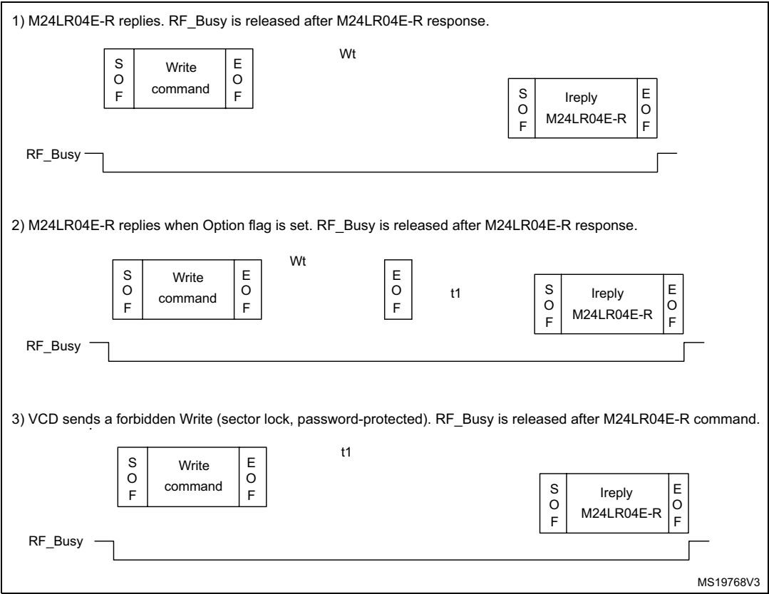
Figure 56. M24LR04E-R RF_Busy management following Write command
