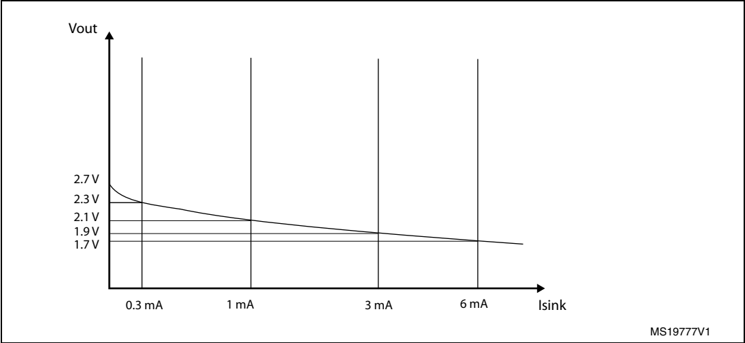
Figure 82. Vout vs. Isink
