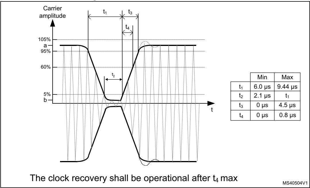
Figure 14. 100% modulation waveform
