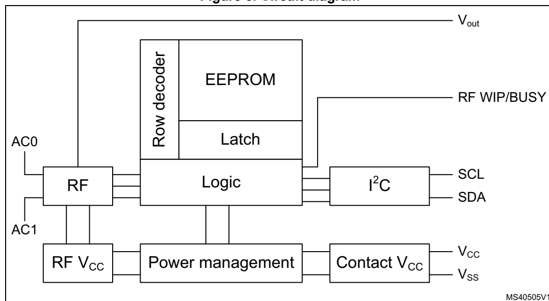
Figure 5. Circuit diagram
