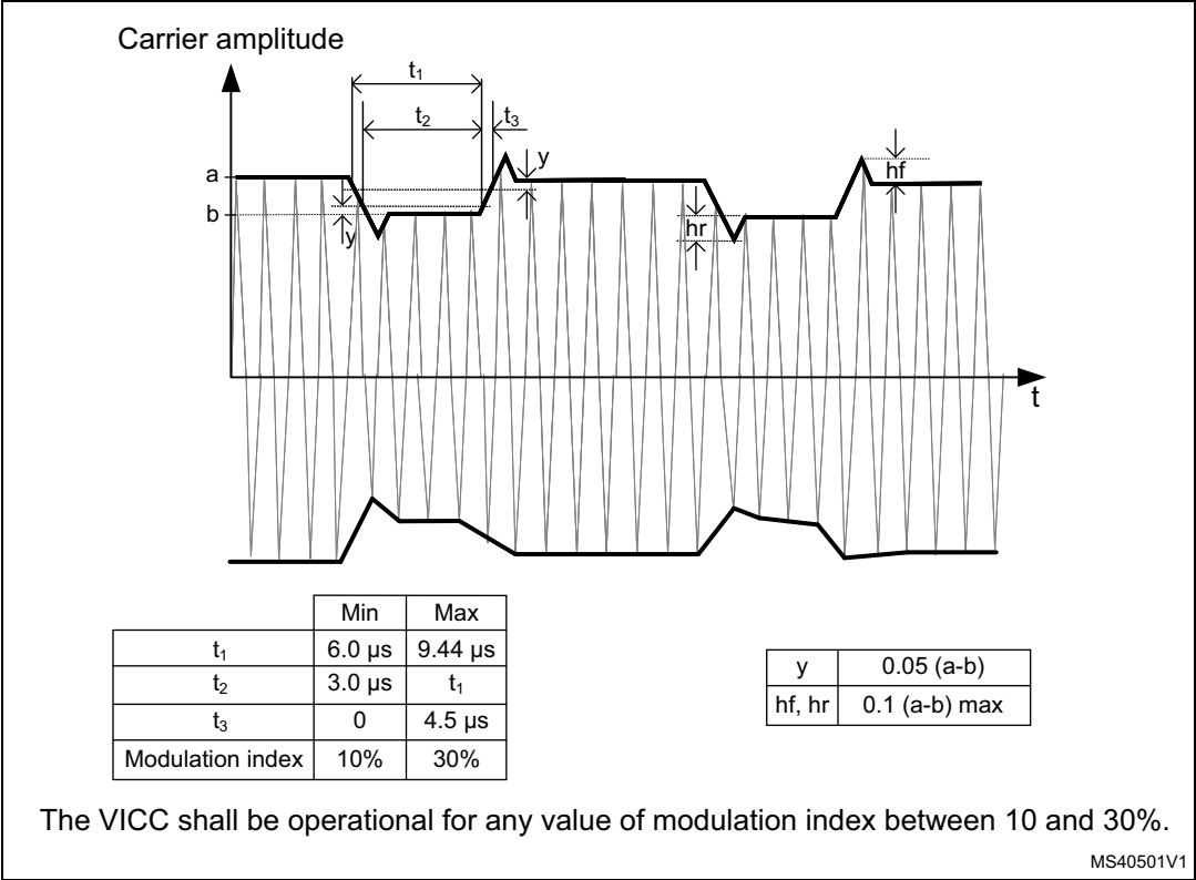
Figure 15. 10% modulation waveform
