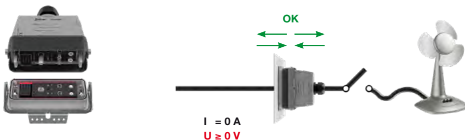
With protection wall
