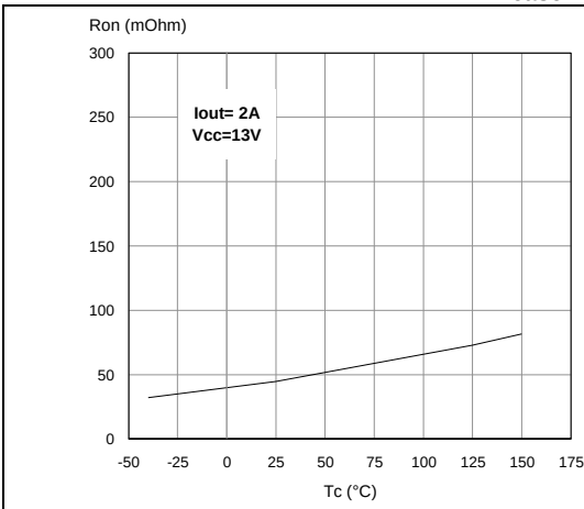
Figure 23. On-state resistance vs T_{case}
