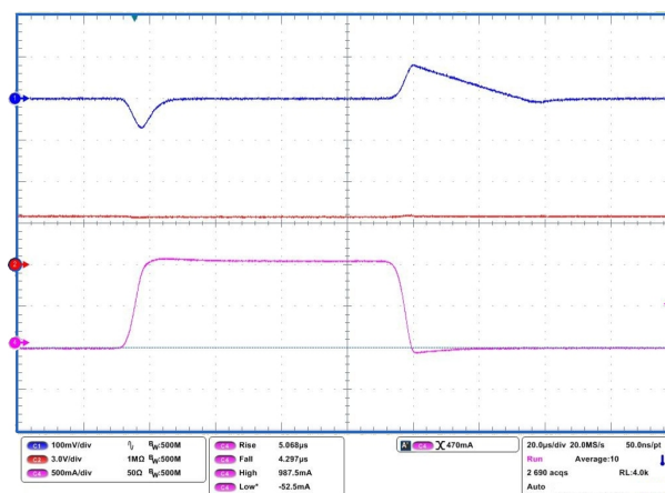
Figure 27. Load transient ( V_{OUT} = 1.2\text{ V} )
