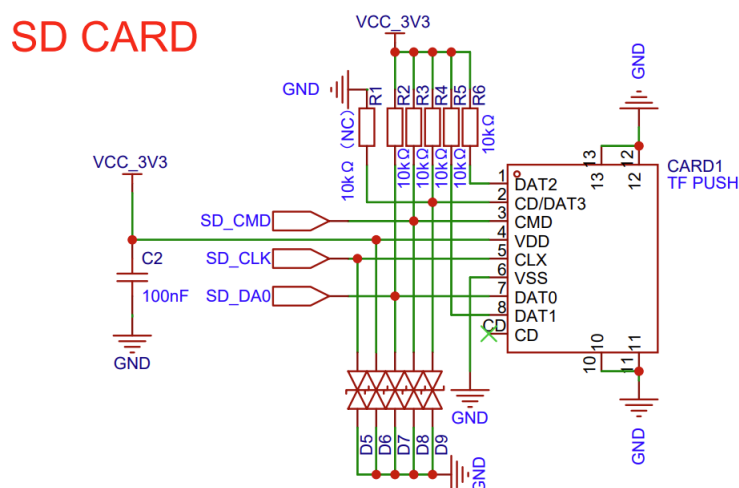
Fig. 16: SD Card Interface Circuit Diagram (Click to enlarge)
