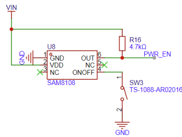
Fig. 37: Power Switch Circuit Diagram (Click to enlarge)
