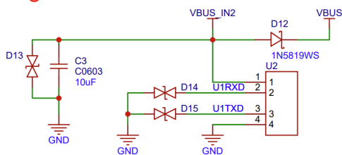
Fig. 34: Magnetic Connector Interface Circuit Diagram (Click to enlarge)
