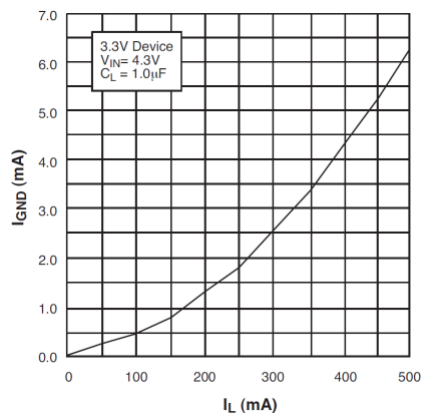
Fig. 3: Ground Current vs Load Current
