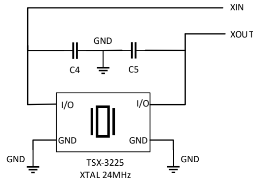
Figure 9.2. External XTAL schematics.
