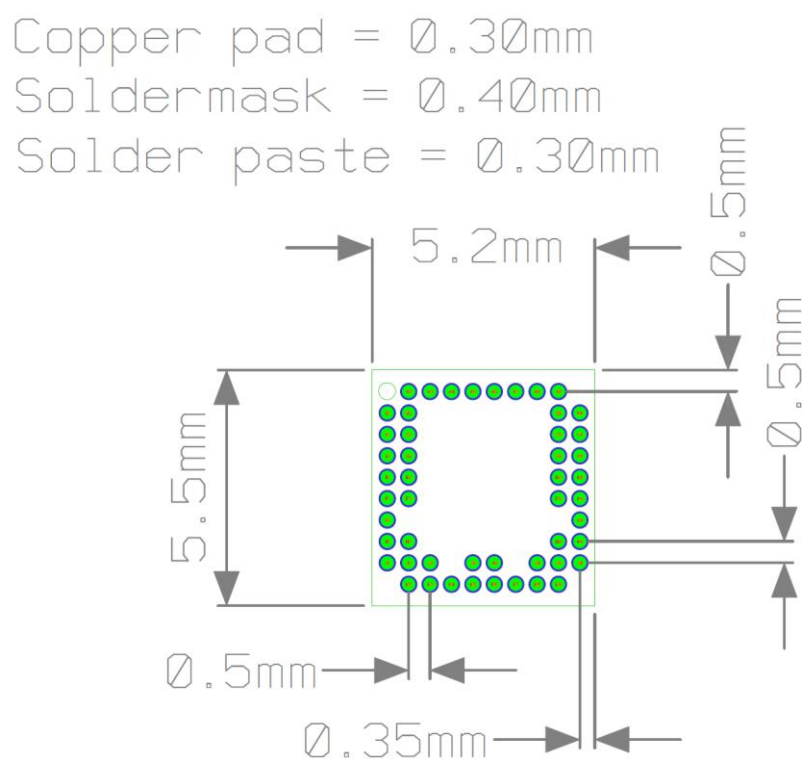
Figure 11.1. A111 footprint.
