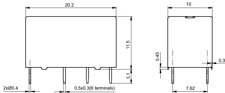
Outline Dimensions
