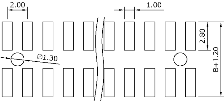
Recommended PCB Layout (PCB TOLERANCE ±0.05)
