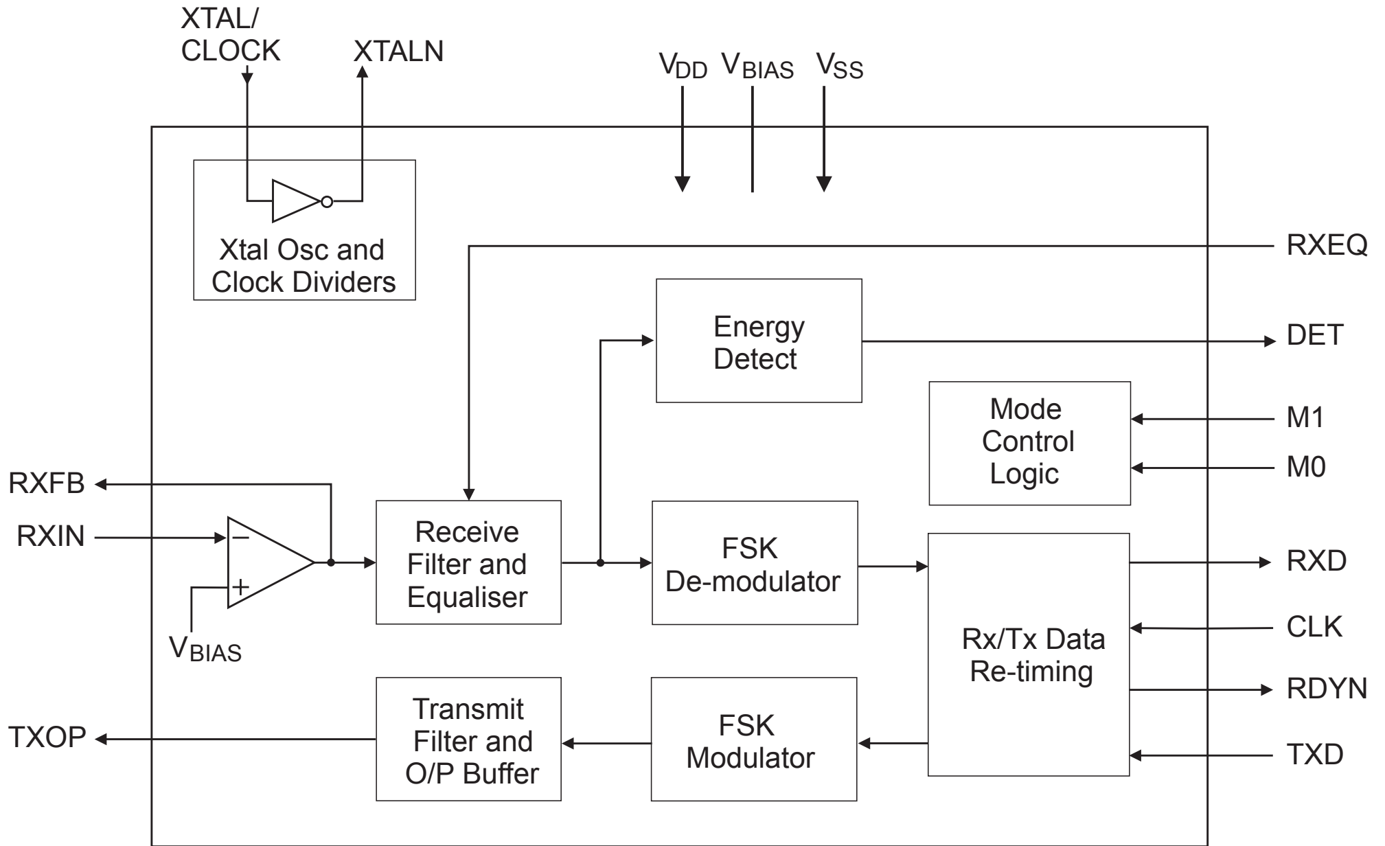
FX/MX614 Block Diagram
