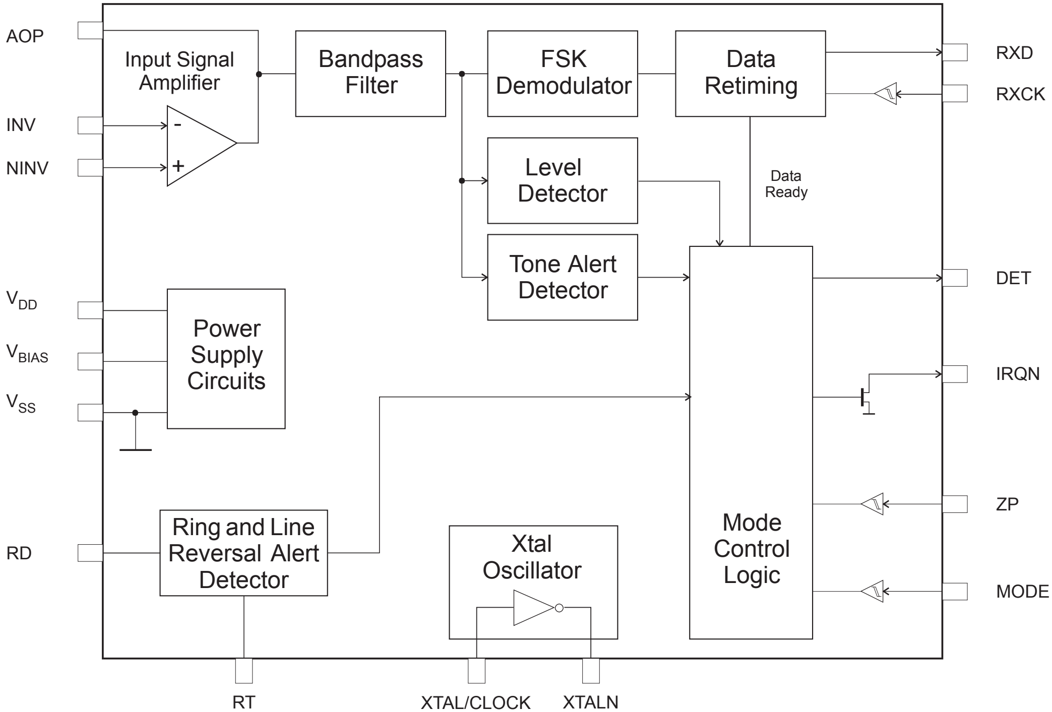
CMX602B Block Diagram
