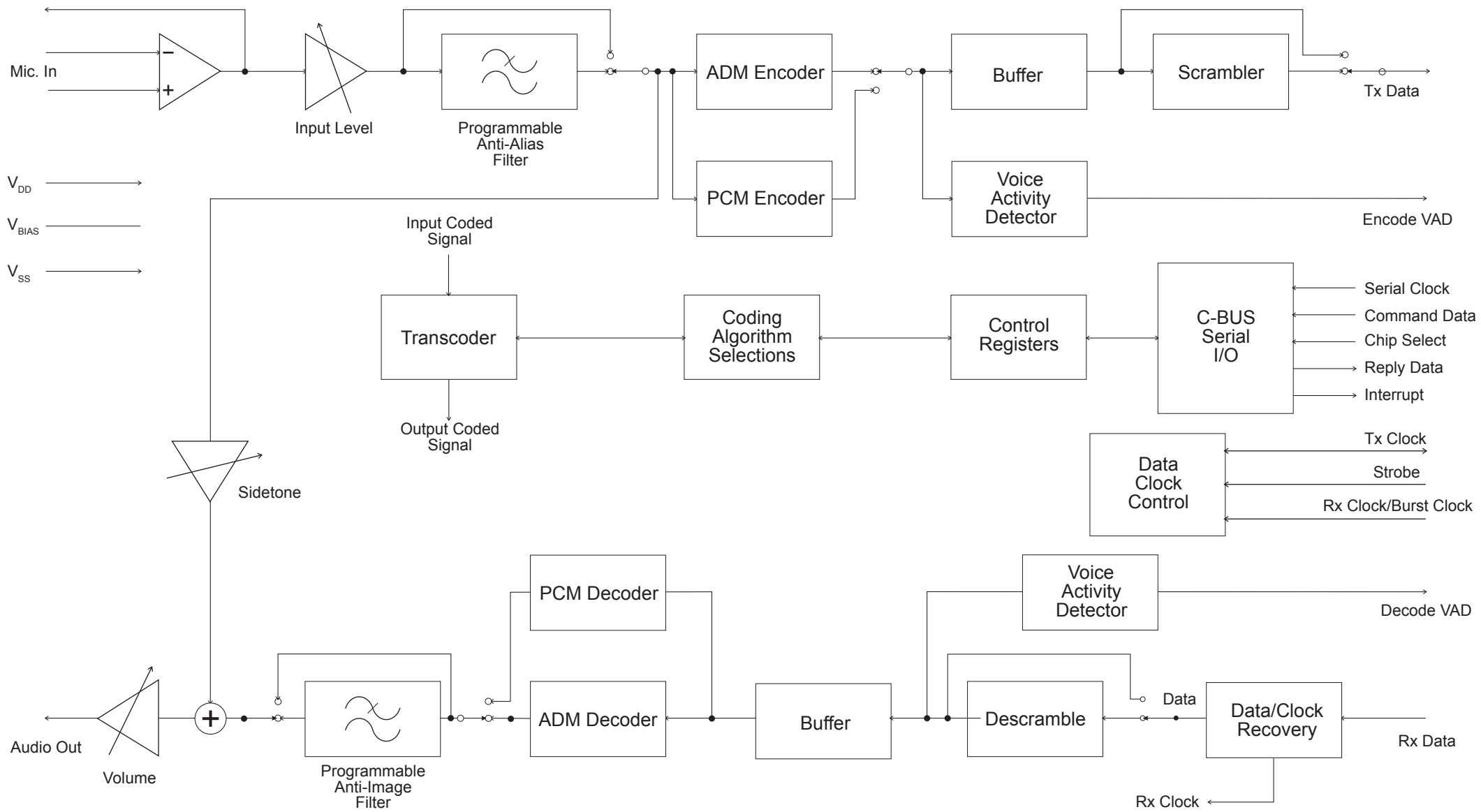
CMX649 Block Diagram
