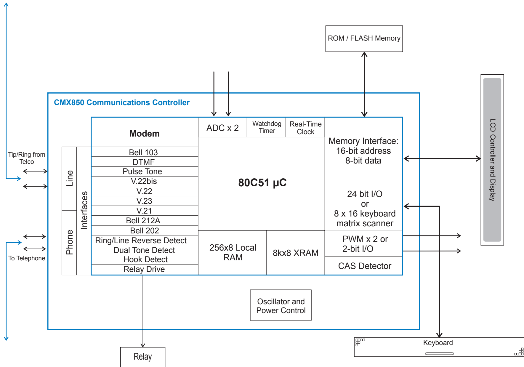
CMX850 Block Diagram
